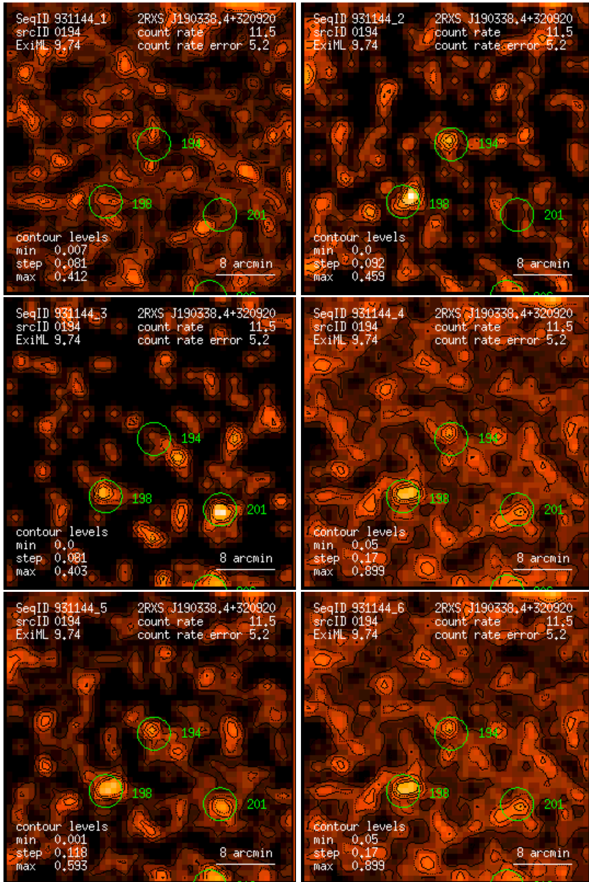
Figure 194: RASS 931144: detection 0194: band rate images, Gaussian filter: (1) PSPC channels 11 – 41, (2) 52 – 90, (3) 91 – 201, (4) 11 – 235, (5) 52 – 201, (6) 11 – 201. Broad band rates in counts/ks. Band rate contour levels in counts/ks/arcmin 2 .
