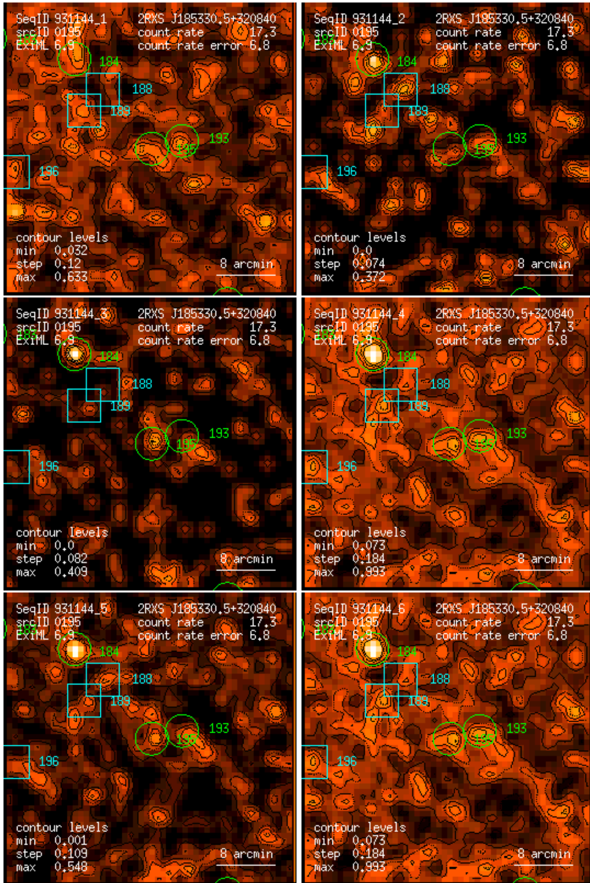
Figure 195: RASS 931144: detection 0195: band rate images, Gaussian filter: (1) PSPC channels 11 – 41, (2) 52 – 90, (3) 91 – 201, (4) 11 – 235, (5) 52 – 201, (6) 11 – 201. Broad band rates in counts/ks. Band rate contour levels in counts/ks/arcmin 2 .
