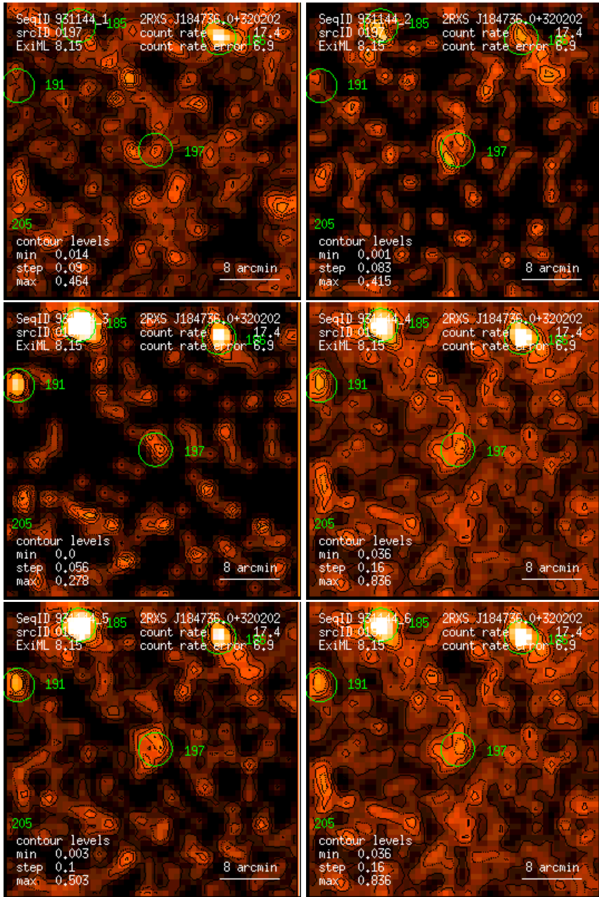
Figure 197: RASS 931144: detection 0197: band rate images, Gaussian filter: (1) PSPC channels 11 – 41, (2) 52 – 90, (3) 91 – 201, (4) 11 – 235, (5) 52 – 201, (6) 11 – 201. Broad band rates in counts/ks. Band rate contour levels in counts/ks/arcmin 2 .
