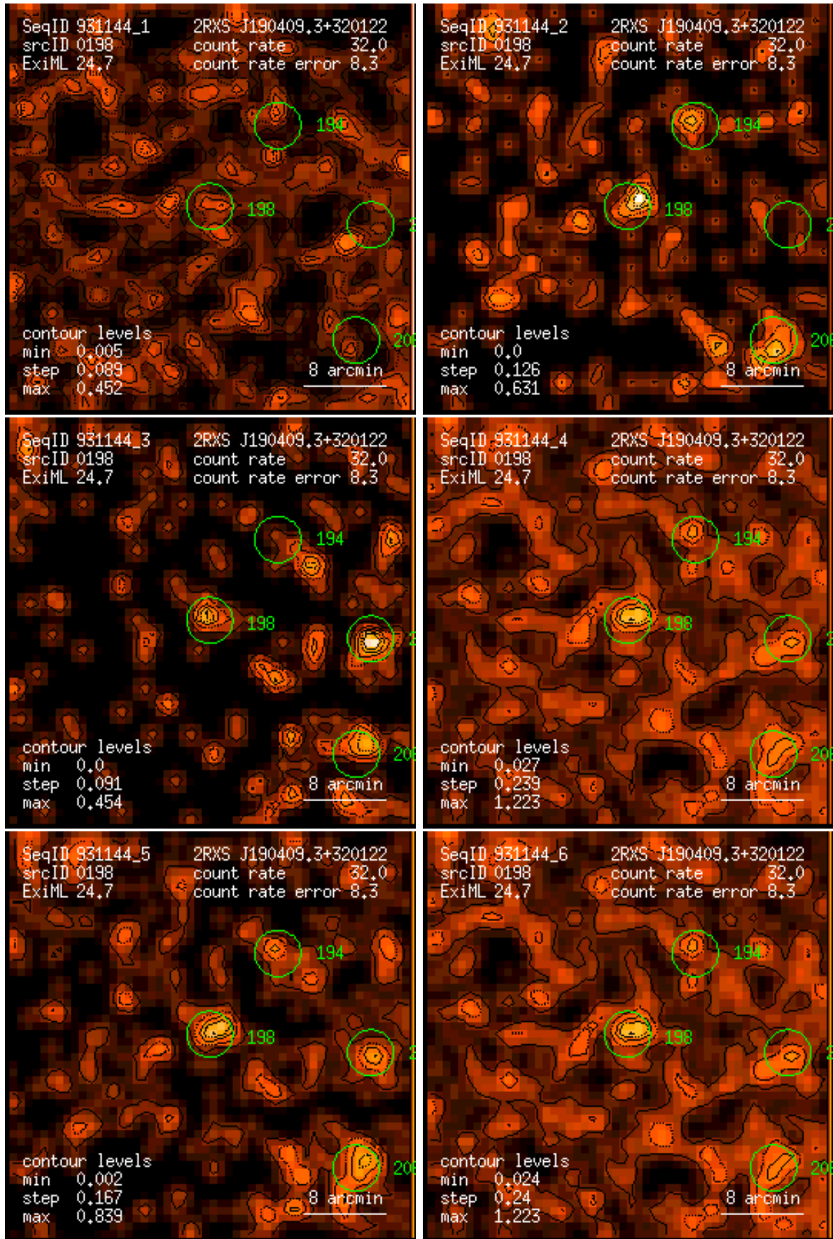
Figure 198: RASS 931144: detection 0198: band rate images, Gaussian filter: (1) PSPC channels 11 – 41, (2) 52 – 90, (3) 91 – 201, (4) 11 – 235, (5) 52 – 201, (6) 11 – 201. Broad band rates in counts/ks. Band rate contour levels in counts/ks/arcmin 2 .
