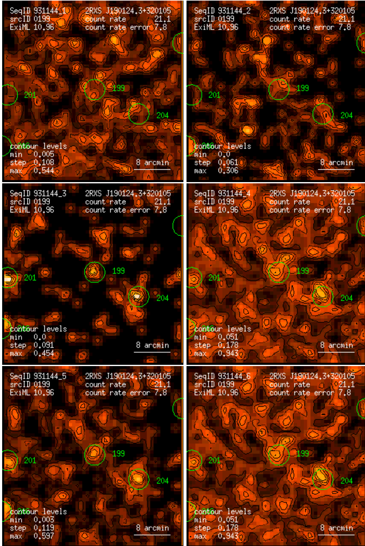
Figure 199: RASS 931144: detection 0199: band rate images, Gaussian filter: (1) PSPC channels 11 – 41, (2) 52 – 90, (3) 91 – 201, (4) 11 – 235, (5) 52 – 201, (6) 11 – 201. Broad band rates in counts/ks. Band rate contour levels in counts/ks/arcmin 2 .
