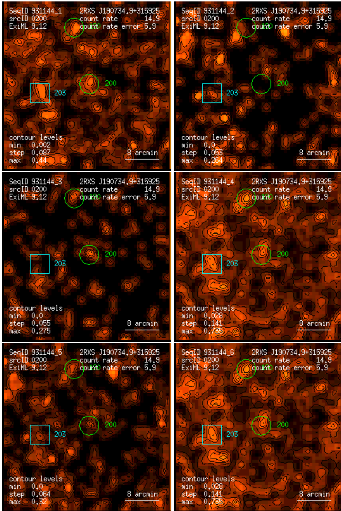
Figure 200: RASS 931144: detection 0200: band rate images, Gaussian filter: (1) PSPC channels 11 – 41, (2) 52 – 90, (3) 91 – 201, (4) 11 – 235, (5) 52 – 201, (6) 11 – 201. Broad band rates in counts/ks. Band rate contour levels in counts/ks/arcmin 2 .
