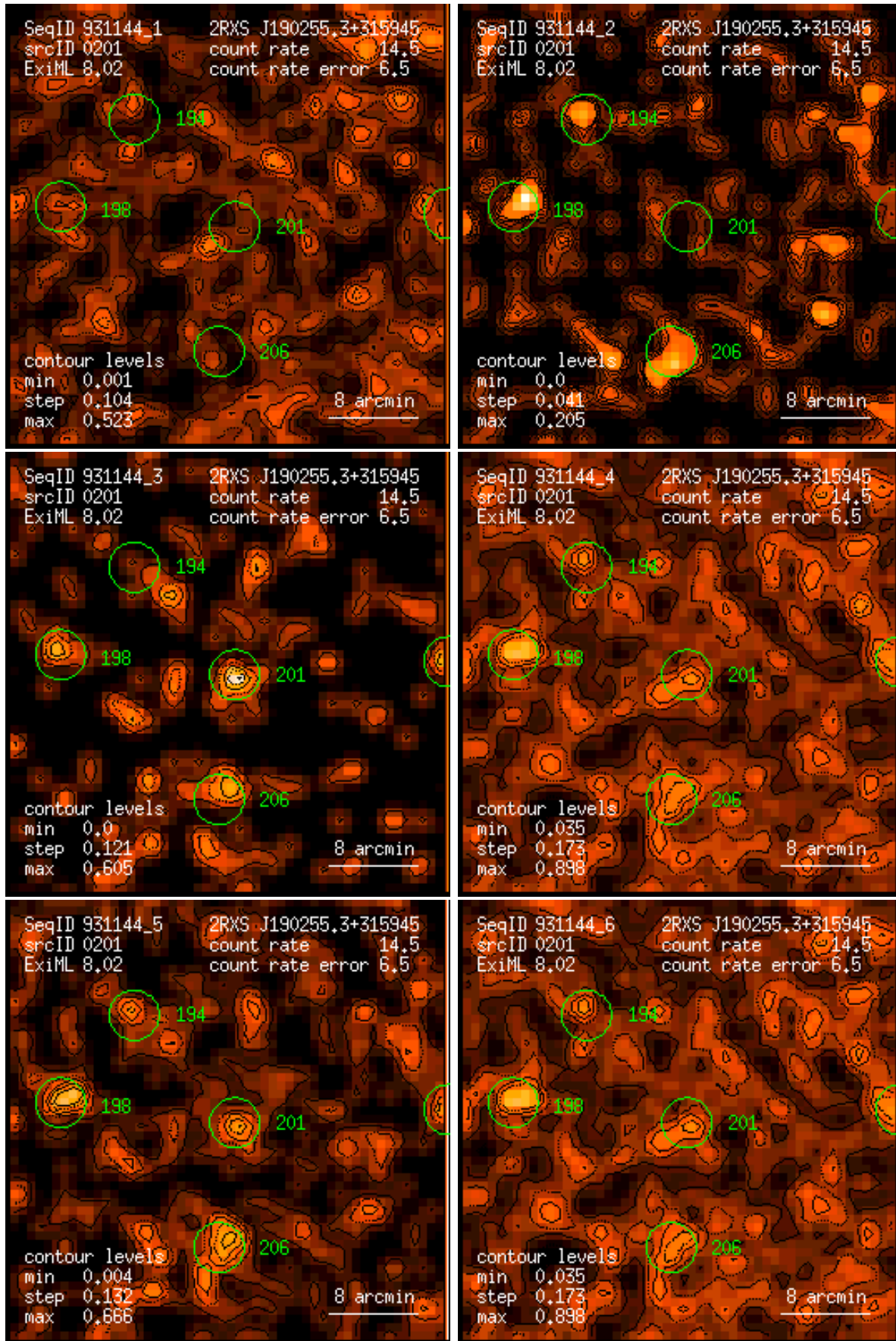
Figure 201: RASS 931144: detection 0201: band rate images, Gaussian filter: (1) PSPC channels 11 – 41, (2) 52 – 90, (3) 91 – 201, (4) 11 – 235, (5) 52 – 201, (6) 11 – 201. Broad band rates in counts/ks. Band rate contour levels in counts/ks/arcmin 2 .
