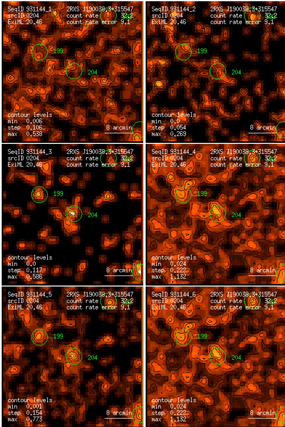
Figure 204: RASS 931144: detection 0204: band rate images, Gaussian filter: (1) PSPC channels 11 – 41, (2) 52 – 90, (3) 91 – 201, (4) 11 – 235, (5) 52 – 201, (6) 11 – 201. Broad band rates in counts/ks. Band rate contour levels in counts/ks/arcmin 2 .
