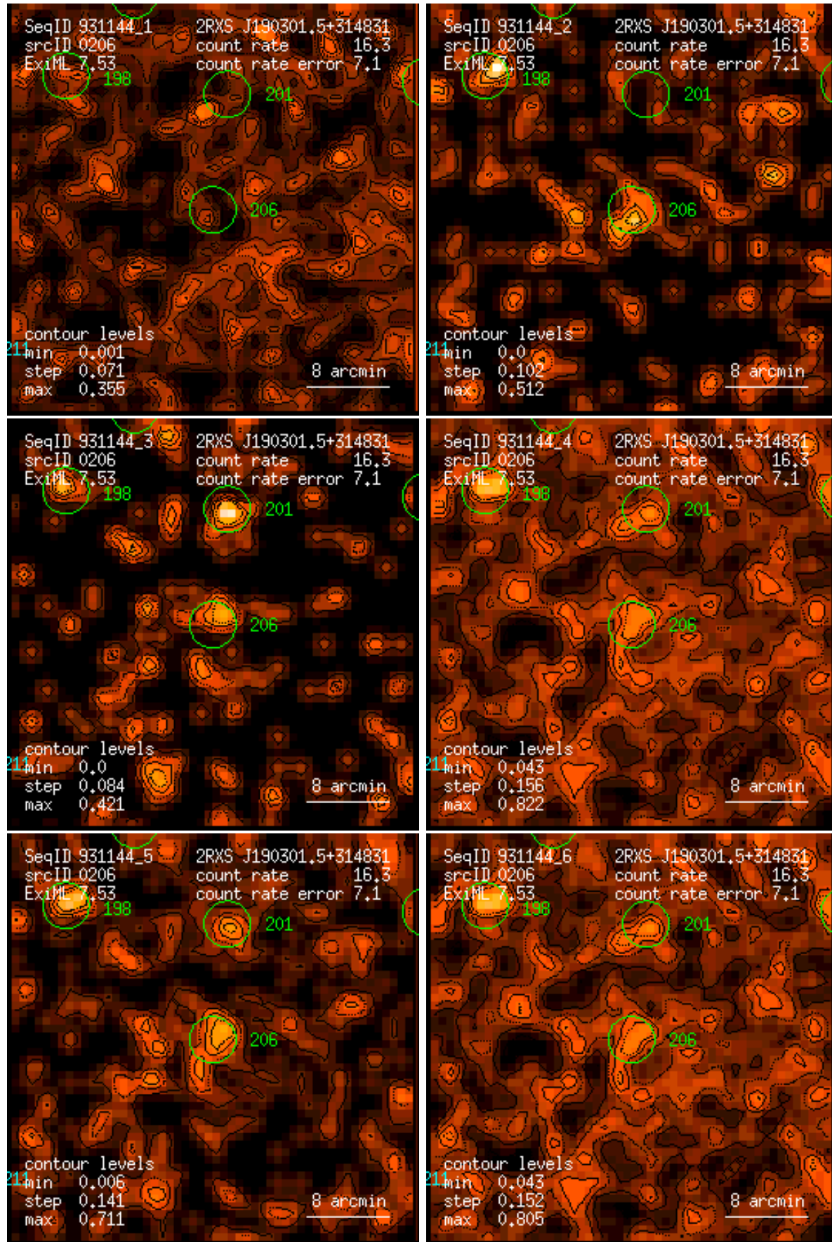
Figure 206: RASS 931144: detection 0206: band rate images, Gaussian filter: (1) PSPC channels 11 – 41, (2) 52 – 90, (3) 91 – 201, (4) 11 – 235, (5) 52 – 201, (6) 11 – 201. Broad band rates in counts/ks. Band rate contour levels in counts/ks/arcmin 2 .
