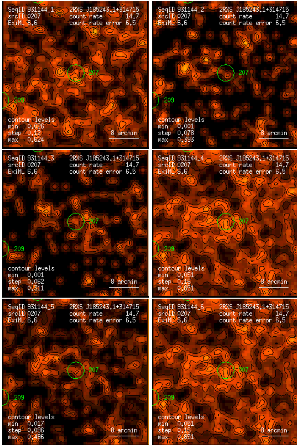
Figure 207: RASS 931144: detection 0207: band rate images, Gaussian filter: (1) PSPC channels 11 – 41, (2) 52 – 90, (3) 91 – 201, (4) 11 – 235, (5) 52 – 201, (6) 11 – 201. Broad band rates in counts/ks. Band rate contour levels in counts/ks/arcmin 2 .
