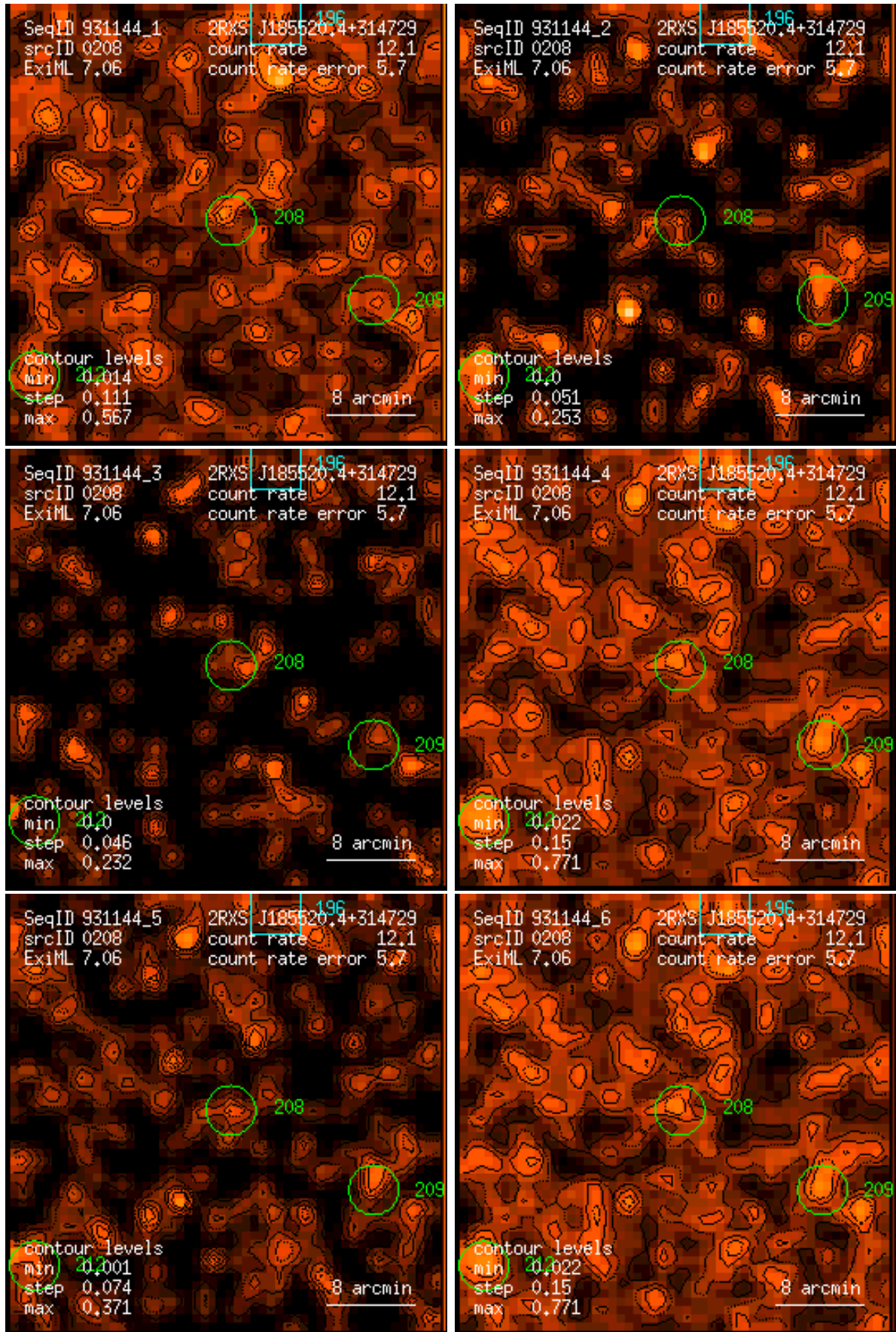
Figure 208: RASS 931144: detection 0208: band rate images, Gaussian filter: (1) PSPC channels 11 – 41, (2) 52 – 90, (3) 91 – 201, (4) 11 – 235, (5) 52 – 201, (6) 11 – 201. Broad band rates in counts/ks. Band rate contour levels in counts/ks/arcmin 2 .
