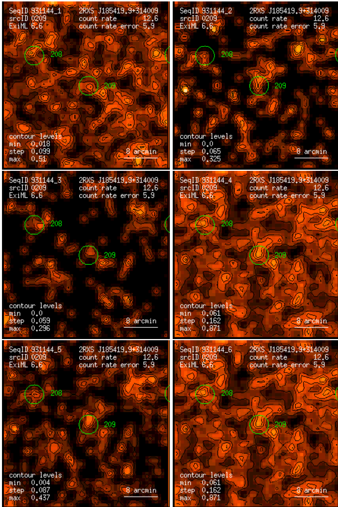
Figure 209: RASS 931144: detection 0209: band rate images, Gaussian filter: (1) PSPC channels 11 – 41, (2) 52 – 90, (3) 91 – 201, (4) 11 – 235, (5) 52 – 201, (6) 11 – 201. Broad band rates in counts/ks. Band rate contour levels in counts/ks/arcmin 2 .
