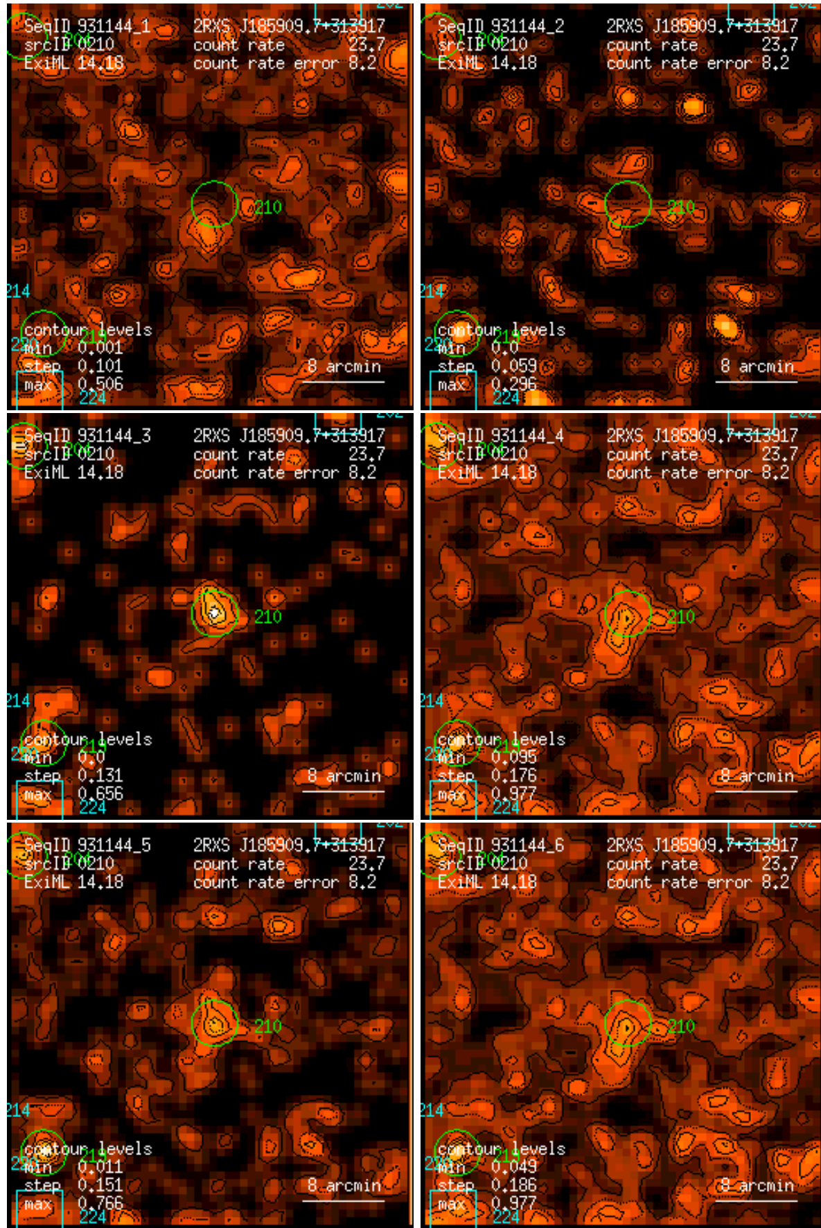
Figure 210: RASS 931144: detection 0210: band rate images, Gaussian filter: (1) PSPC channels 11 – 41, (2) 52 – 90, (3) 91 – 201, (4) 11 – 235, (5) 52 – 201, (6) 11 – 201. Broad band rates in counts/ks. Band rate contour levels in counts/ks/arcmin 2 .
