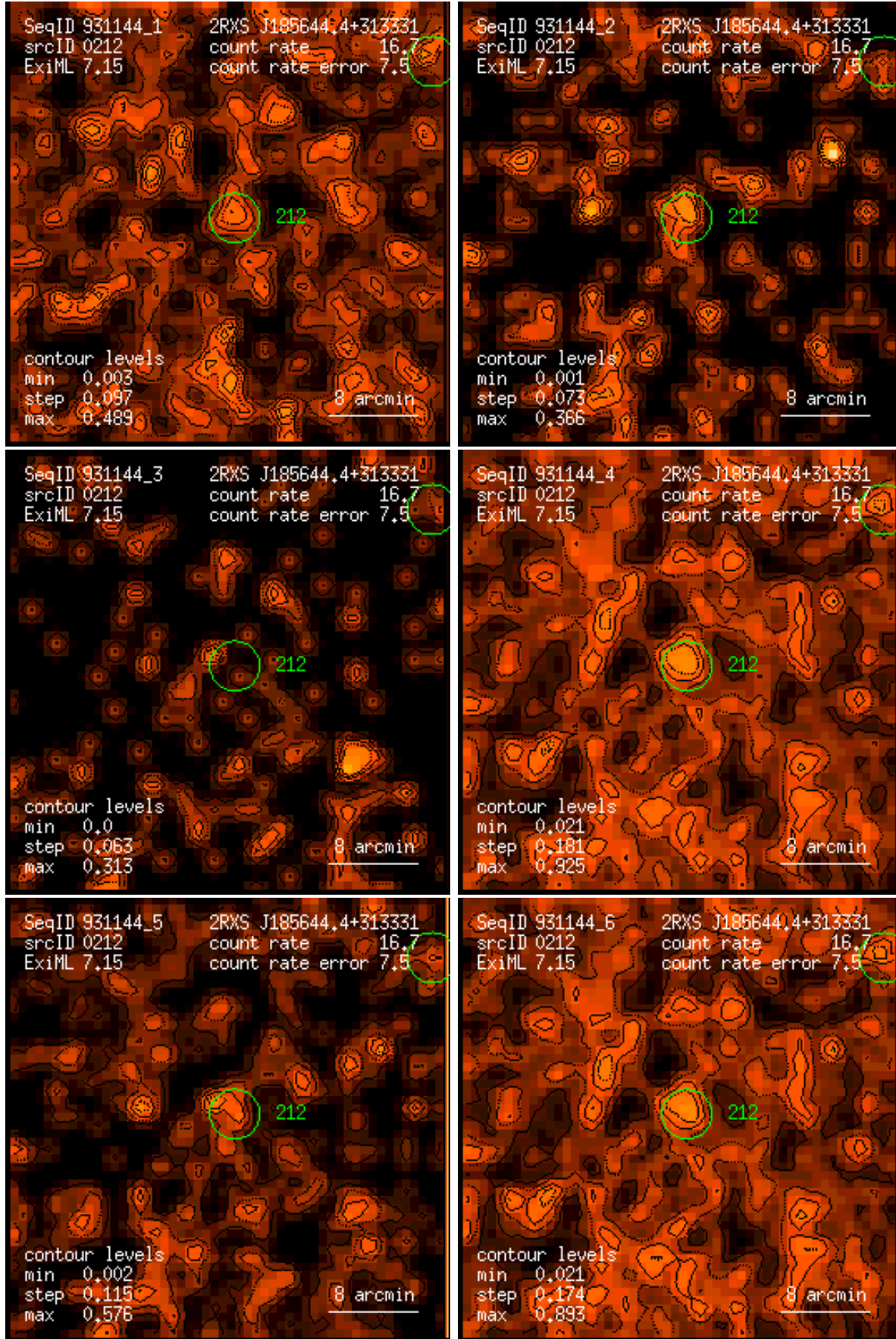
Figure 212: RASS 931144: detection 0212: band rate images, Gaussian filter: (1) PSPC channels 11 – 41, (2) 52 – 90, (3) 91 – 201, (4) 11 – 235, (5) 52 – 201, (6) 11 – 201. Broad band rates in counts/ks. Band rate contour levels in counts/ks/arcmin 2 .
