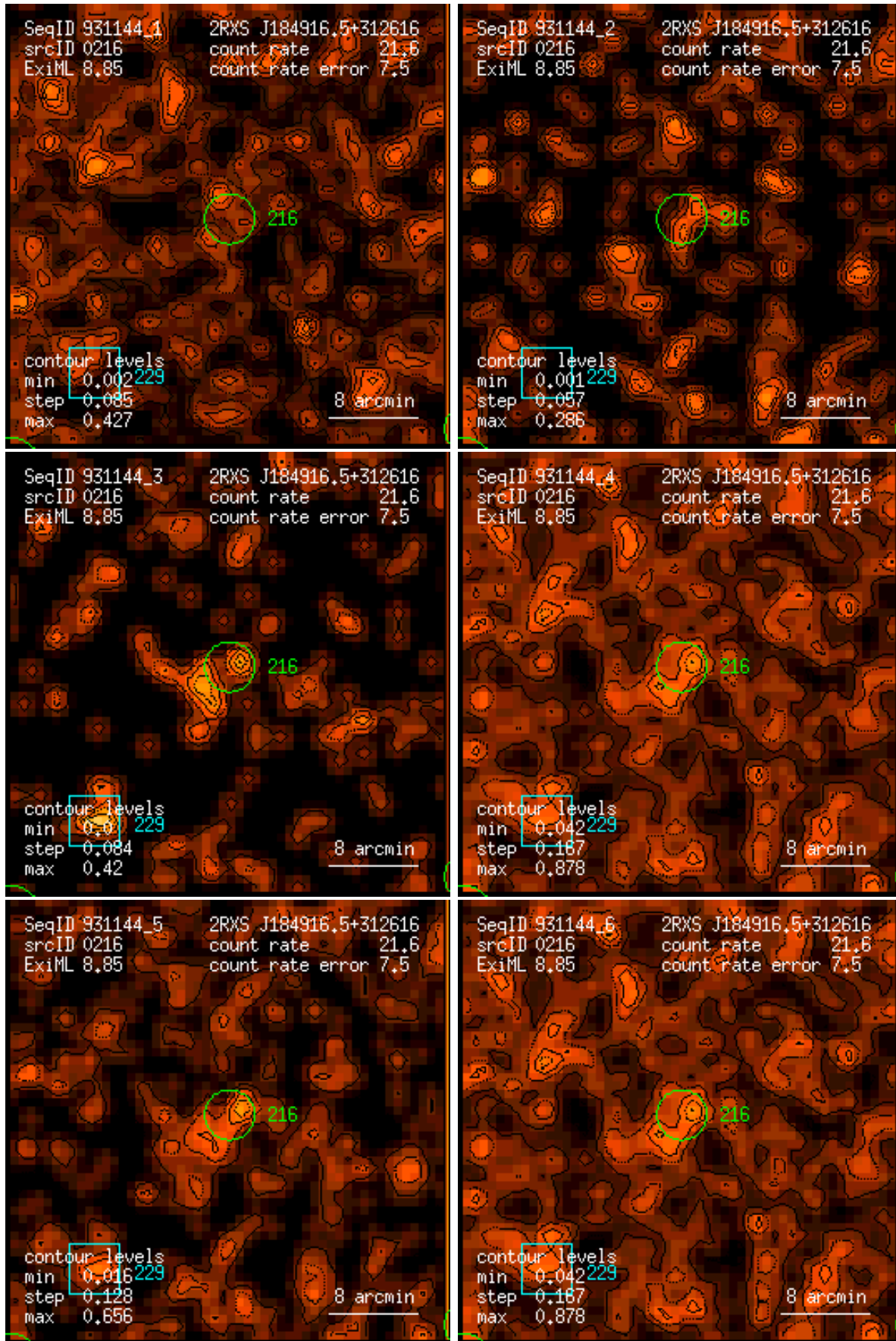
Figure 216: RASS 931144: detection 0216: band rate images, Gaussian filter: (1) PSPC channels 11 – 41, (2) 52 – 90, (3) 91 – 201, (4) 11 – 235, (5) 52 – 201, (6) 11 – 201. Broad band rates in counts/ks. Band rate contour levels in counts/ks/arcmin 2 .
