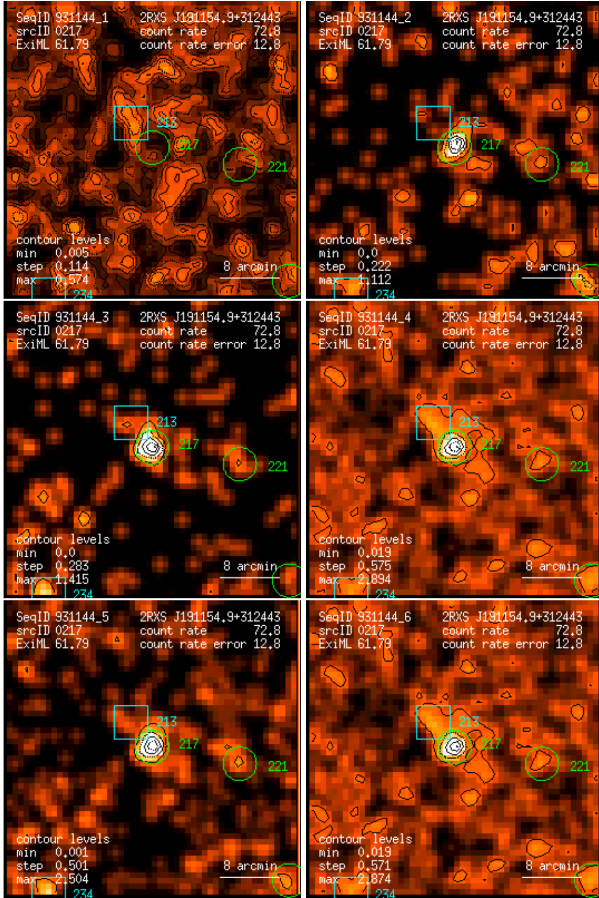
Figure 217: RASS 931144: detection 0217: band rate images, Gaussian filter: (1) PSPC channels 11 – 41, (2) 52 – 90, (3) 91 – 201, (4) 11 – 235, (5) 52 – 201, (6) 11 – 201. Broad band rates in counts/ks. Band rate contour levels in counts/ks/arcmin 2 .
