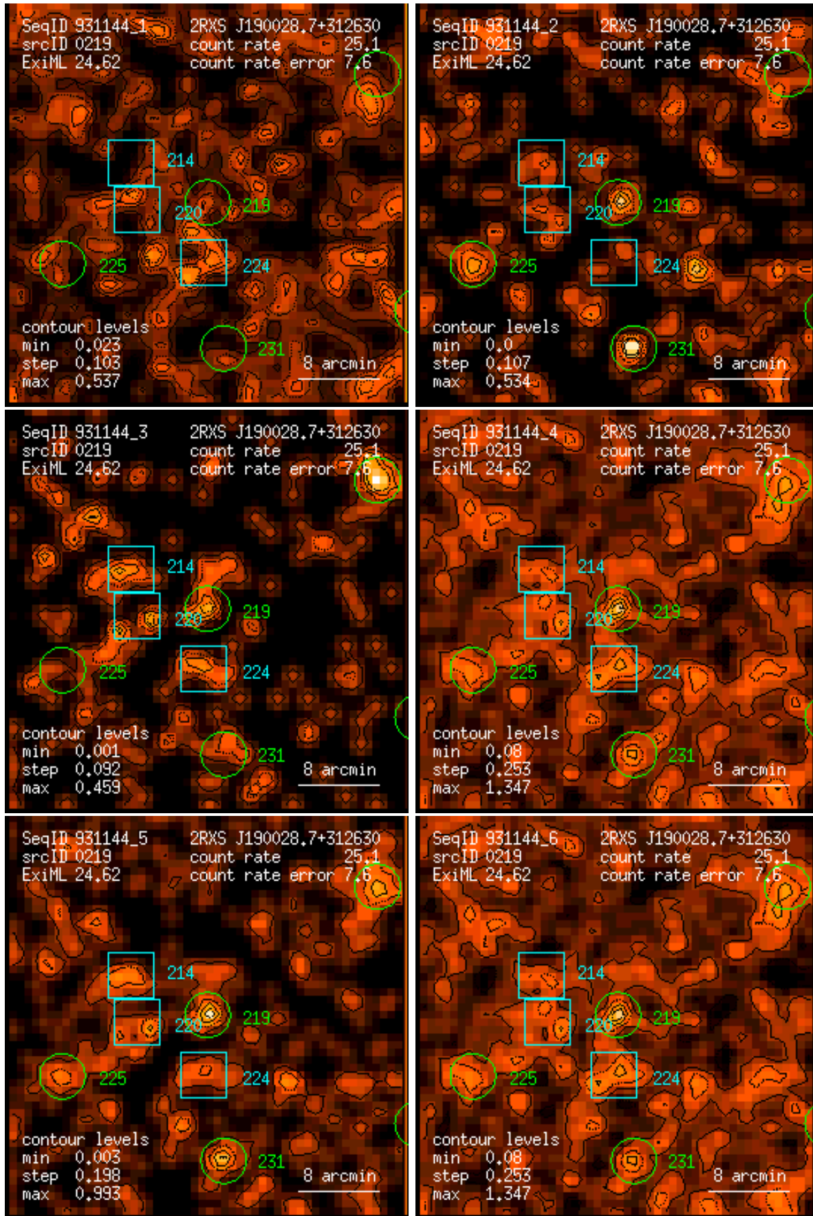
Figure 219: RASS 931144: detection 0219: band rate images, Gaussian filter: (1) PSPC channels 11 – 41, (2) 52 – 90, (3) 91 – 201, (4) 11 – 235, (5) 52 – 201, (6) 11 – 201. Broad band rates in counts/ks. Band rate contour levels in counts/ks/arcmin 2 .
