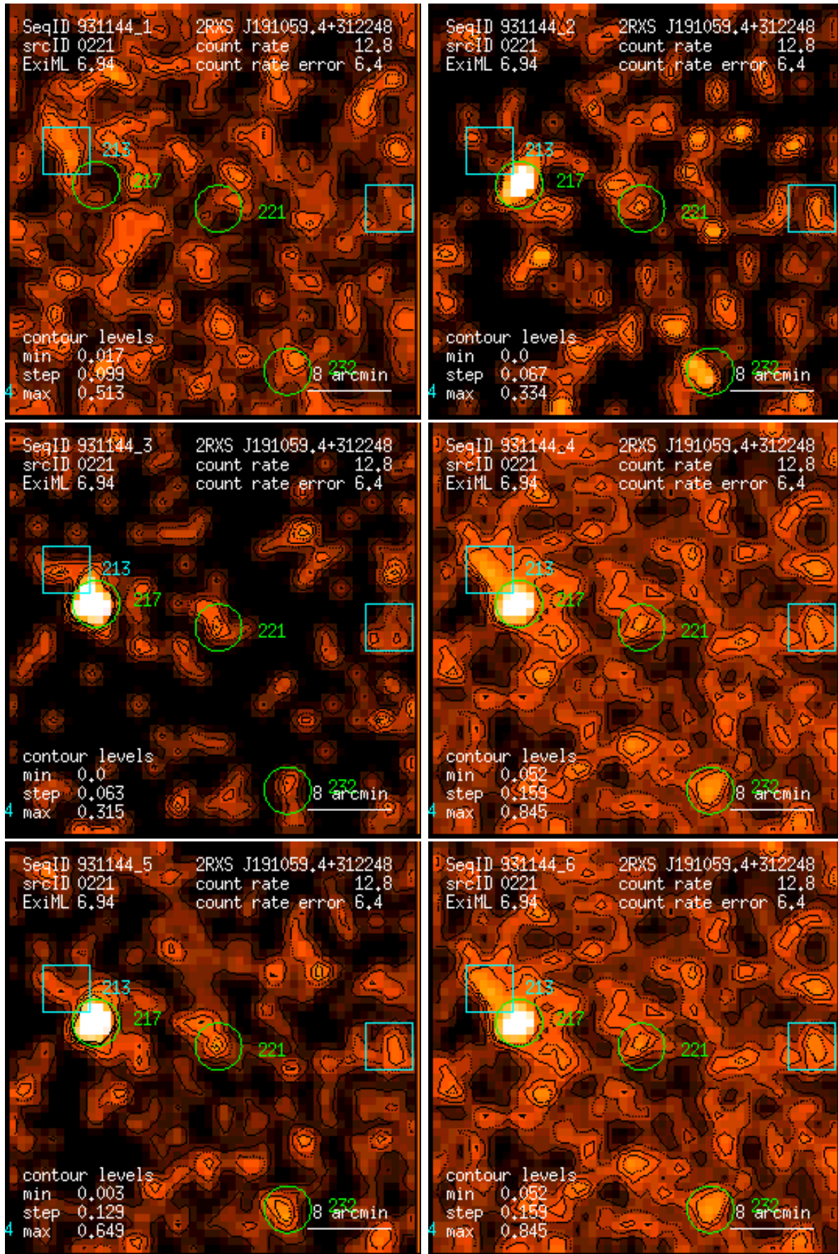
Figure 221: RASS 931144: detection 0221: band rate images, Gaussian filter: (1) PSPC channels 11 – 41, (2) 52 – 90, (3) 91 – 201, (4) 11 – 235, (5) 52 – 201, (6) 11 – 201. Broad band rates in counts/ks. Band rate contour levels in counts/ks/arcmin 2 .
