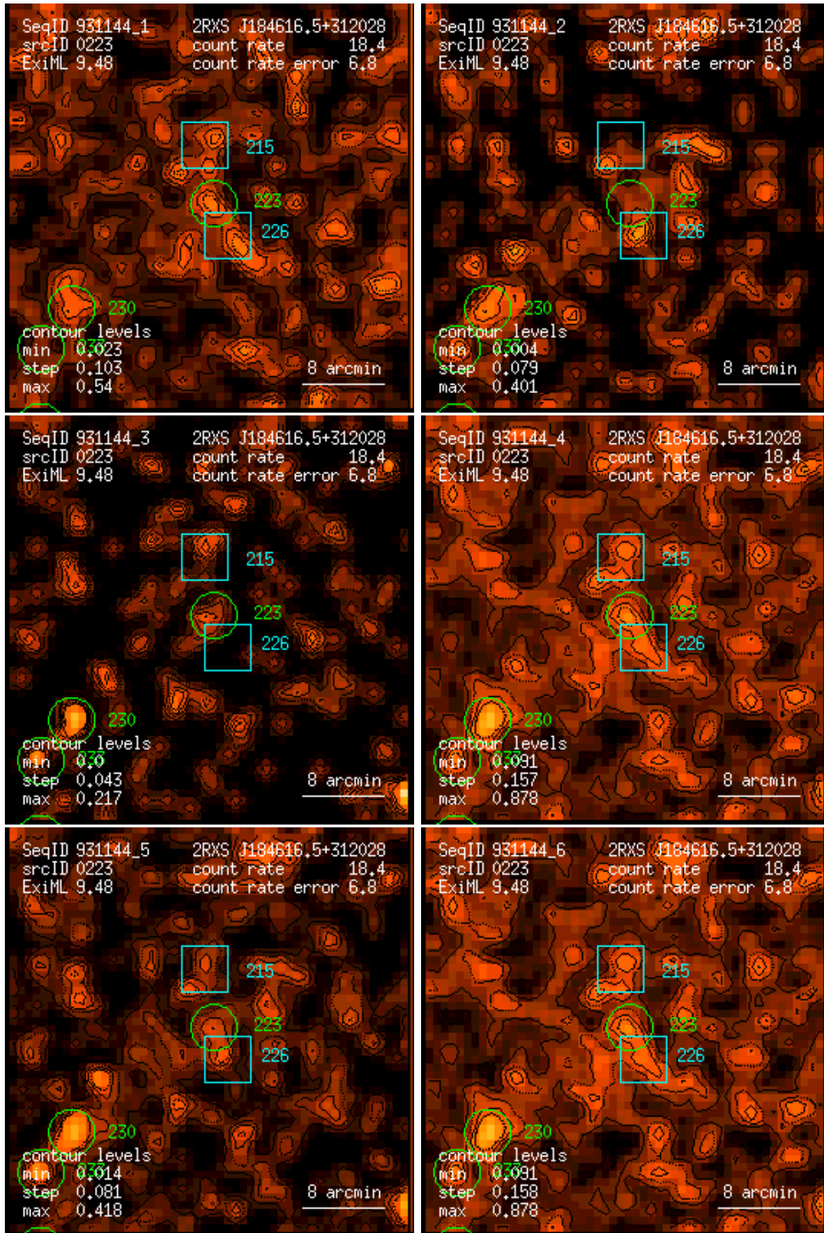
Figure 223: RASS 931144: detection 0223: band rate images, Gaussian filter: (1) PSPC channels 11 – 41, (2) 52 – 90, (3) 91 – 201, (4) 11 – 235, (5) 52 – 201, (6) 11 – 201. Broad band rates in counts/ks. Band rate contour levels in counts/ks/arcmin 2 .
