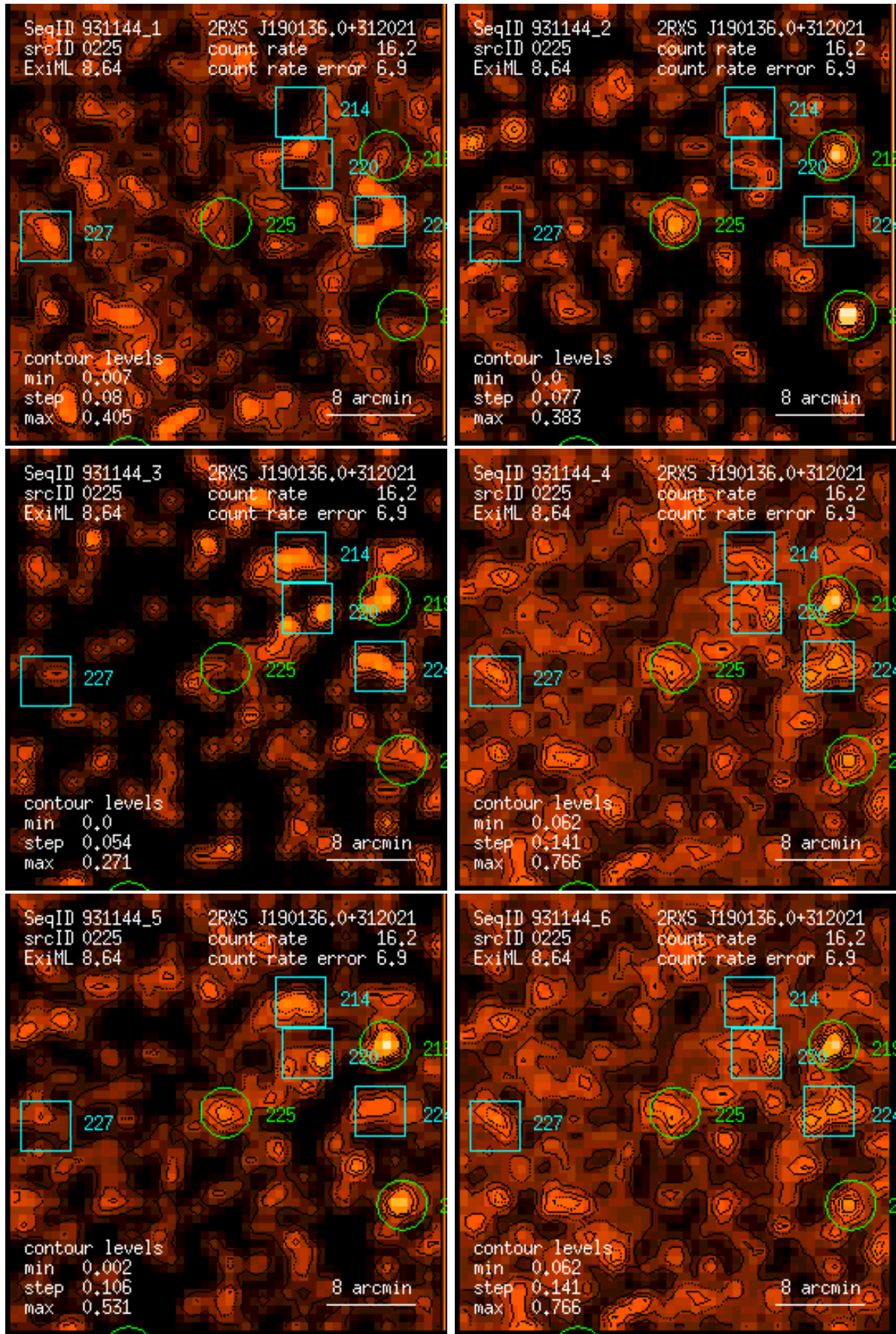
Figure 225: RASS 931144: detection 0225: band rate images, Gaussian filter: (1) PSPC channels 11 – 41, (2) 52 – 90, (3) 91 – 201, (4) 11 – 235, (5) 52 – 201, (6) 11 – 201. Broad band rates in counts/ks. Band rate contour levels in counts/ks/arcmin 2 .
