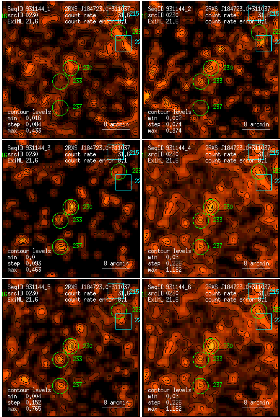
Figure 230: RASS 931144: detection 0230: band rate images, Gaussian filter: (1) PSPC channels 11 – 41, (2) 52 – 90, (3) 91 – 201, (4) 11 – 235, (5) 52 – 201, (6) 11 – 201. Broad band rates in counts/ks. Band rate contour levels in counts/ks/arcmin 2 .
