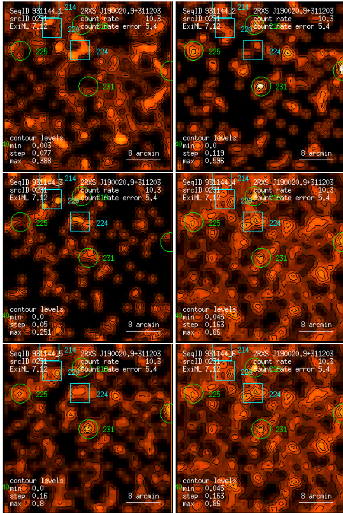
Figure 231: RASS 931144: detection 0231: band rate images, Gaussian filter: (1) PSPC channels 11 – 41, (2) 52 – 90, (3) 91 – 201, (4) 11 – 235, (5) 52 – 201, (6) 11 – 201. Broad band rates in counts/ks. Band rate contour levels in counts/ks/arcmin 2 .
