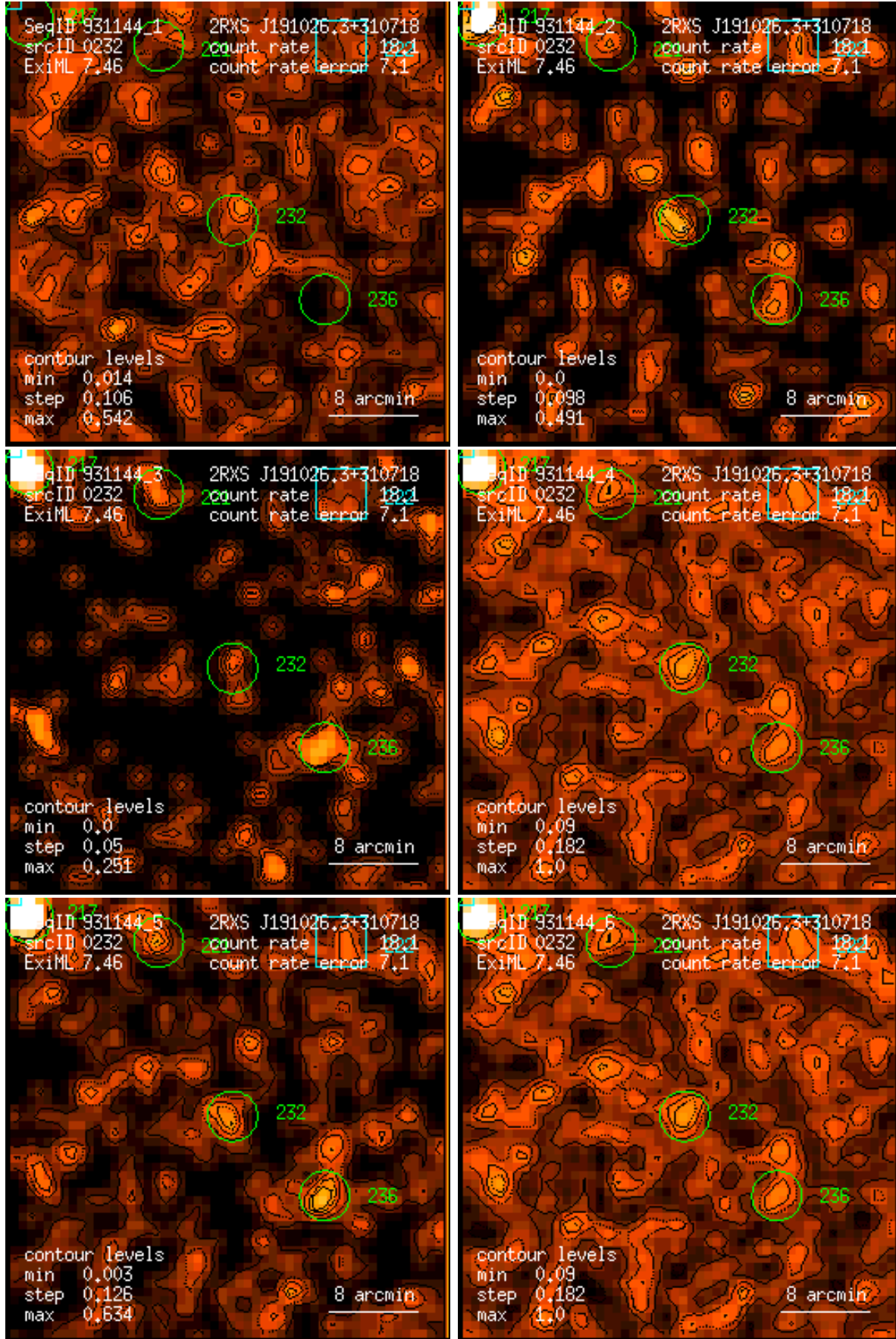
Figure 232: RASS 931144: detection 0232: band rate images, Gaussian filter: (1) PSPC channels 11 – 41, (2) 52 – 90, (3) 91 – 201, (4) 11 – 235, (5) 52 – 201, (6) 11 – 201. Broad band rates in counts/ks. Band rate contour levels in counts/ks/arcmin 2 .
