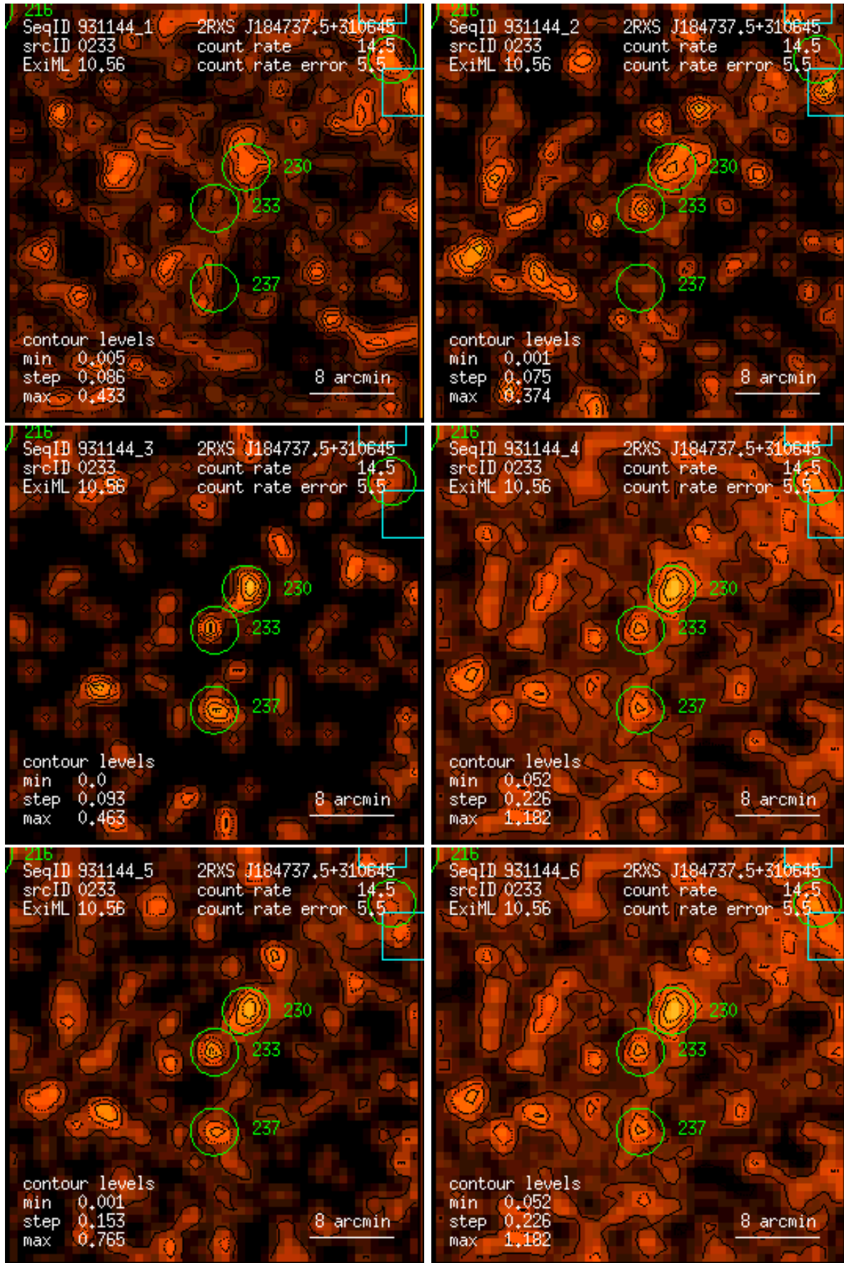
Figure 233: RASS 931144: detection 0233: band rate images, Gaussian filter: (1) PSPC channels 11 – 41, (2) 52 – 90, (3) 91 – 201, (4) 11 – 235, (5) 52 – 201, (6) 11 – 201. Broad band rates in counts/ks. Band rate contour levels in counts/ks/arcmin 2 .
