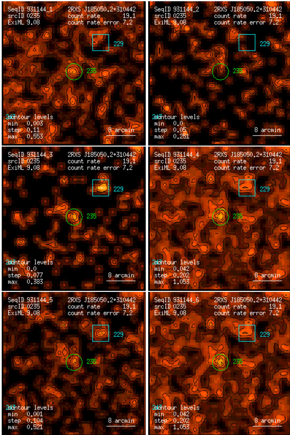
Figure 235: RASS 931144: detection 0235: band rate images, Gaussian filter: (1) PSPC channels 11 – 41, (2) 52 – 90, (3) 91 – 201, (4) 11 – 235, (5) 52 – 201, (6) 11 – 201. Broad band rates in counts/ks. Band rate contour levels in counts/ks/arcmin 2 .
