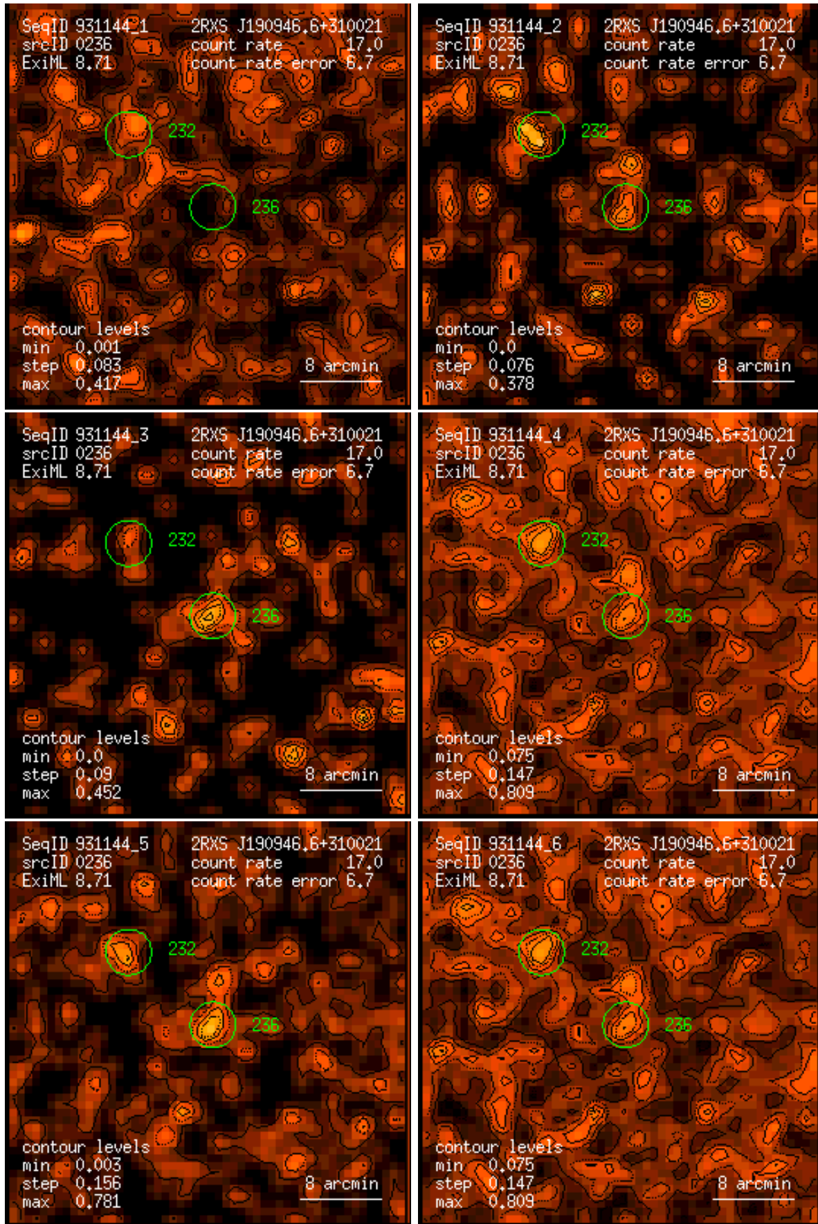
Figure 236: RASS 931144: detection 0236: band rate images, Gaussian filter: (1) PSPC channels 11 – 41, (2) 52 – 90, (3) 91 – 201, (4) 11 – 235, (5) 52 – 201, (6) 11 – 201. Broad band rates in counts/ks. Band rate contour levels in counts/ks/arcmin 2 .
