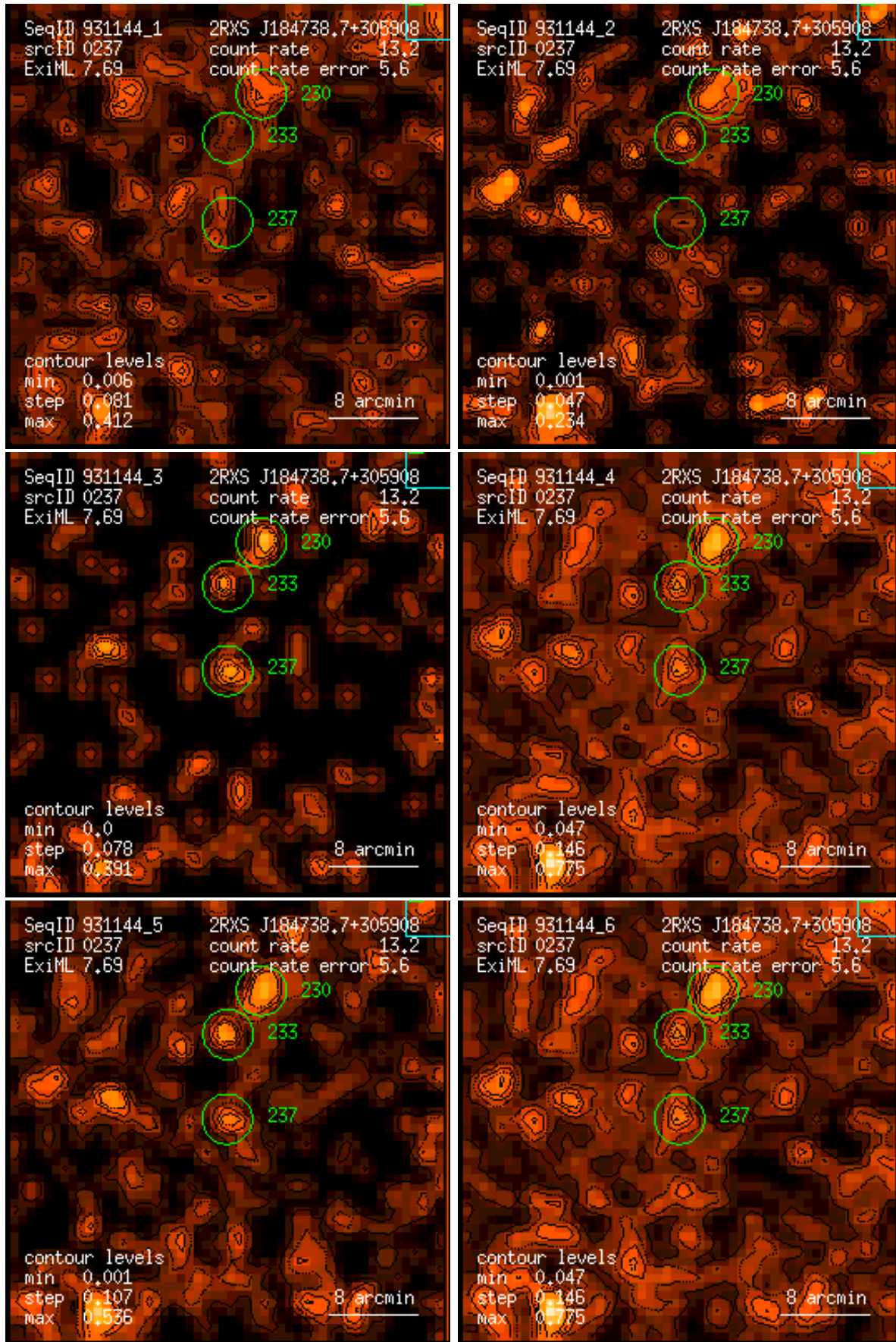
Figure 237: RASS 931144: detection 0237: band rate images, Gaussian filter: (1) PSPC channels 11 – 41, (2) 52 – 90, (3) 91 – 201, (4) 11 – 235, (5) 52 – 201, (6) 11 – 201. Broad band rates in counts/ks. Band rate contour levels in counts/ks/arcmin 2 .
