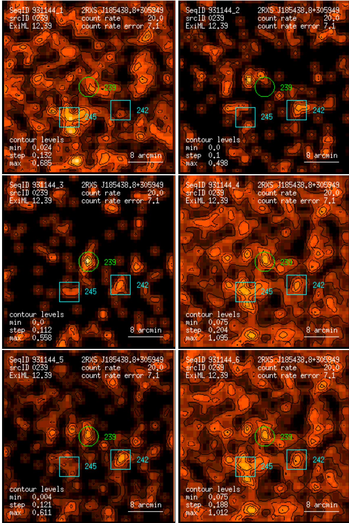
Figure 239: RASS 931144: detection 0239: band rate images, Gaussian filter: (1) PSPC channels 11 – 41, (2) 52 – 90, (3) 91 – 201, (4) 11 – 235, (5) 52 – 201, (6) 11 – 201. Broad band rates in counts/ks. Band rate contour levels in counts/ks/arcmin 2 .
