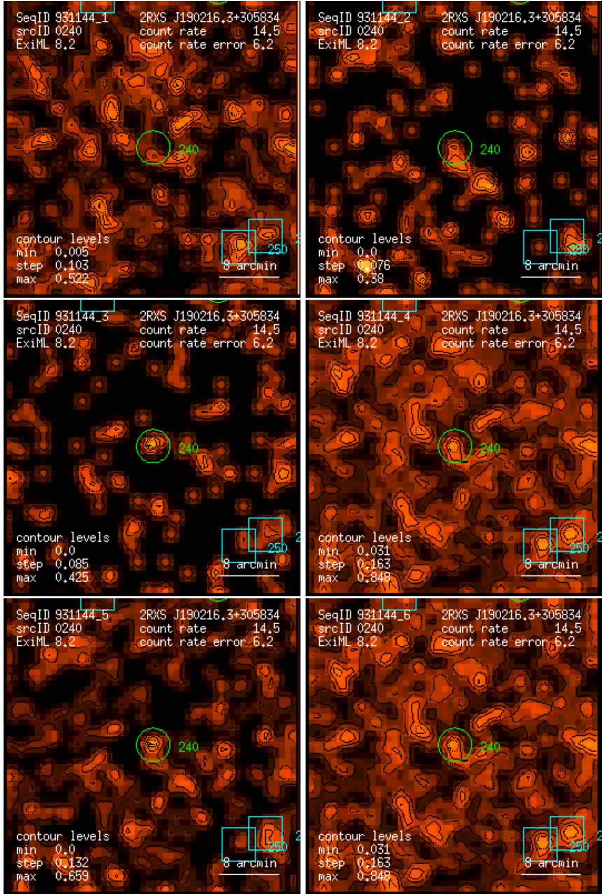
Figure 240: RASS 931144: detection 0240: band rate images, Gaussian filter: (1) PSPC channels 11 – 41, (2) 52 – 90, (3) 91 – 201, (4) 11 – 235, (5) 52 – 201, (6) 11 – 201. Broad band rates in counts/ks. Band rate contour levels in counts/ks/arcmin 2 .
