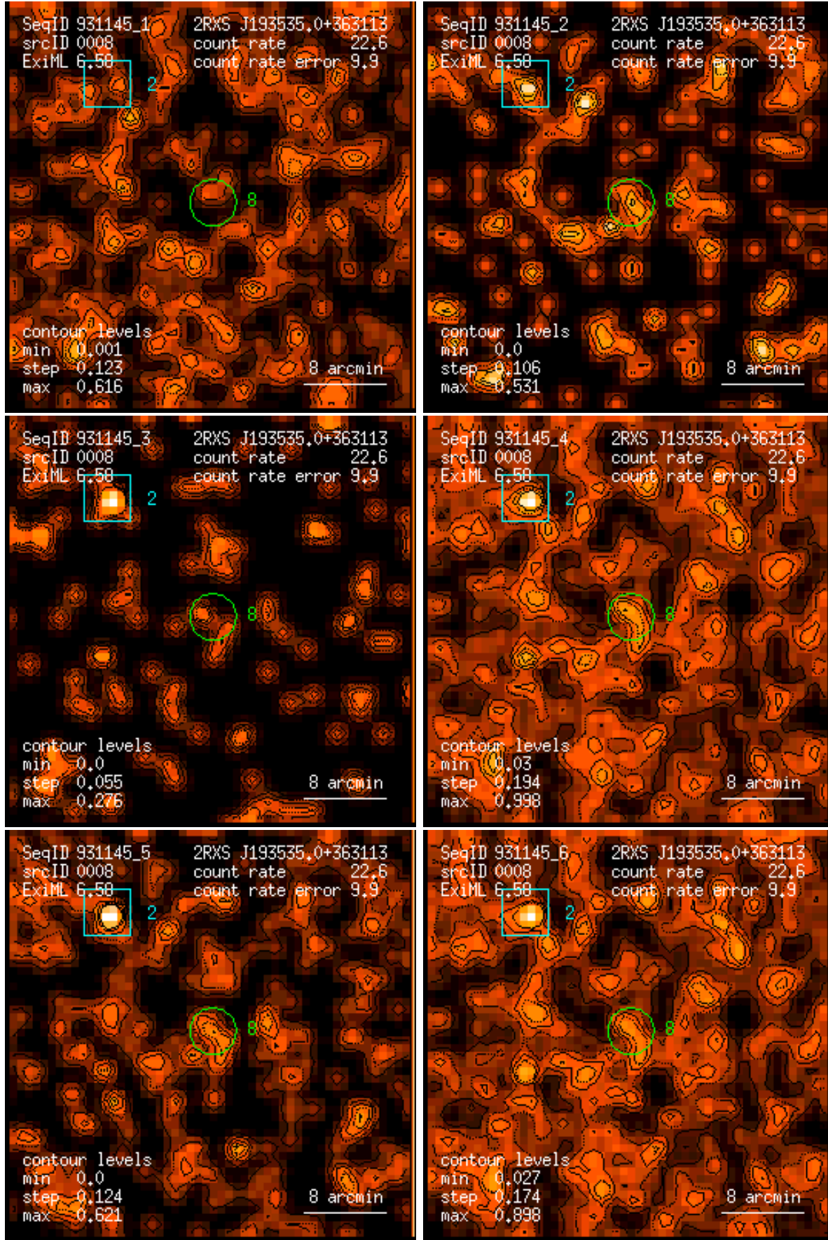
Figure 8: RASS 931145: detection 0008: band rate images, Gaussian filter: (1) PSPC channels 11 – 41, (2) 52 – 90, (3) 91 – 201, (4) 11 – 235, (5) 52 – 201, (6) 11 – 201. Broad band rates in counts/ks. Band rate contour levels in counts/ks/arcmin 2 .
