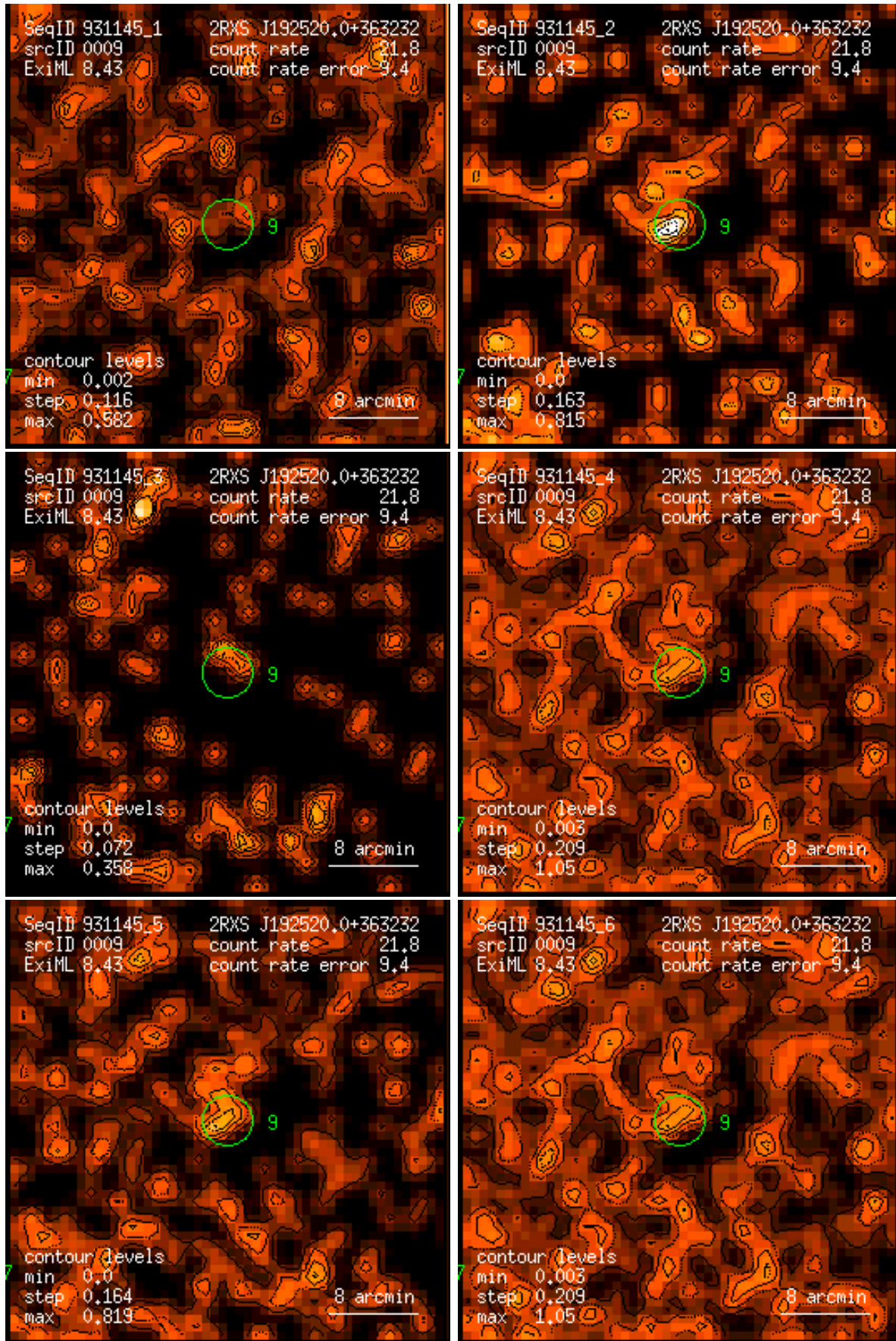
Figure 9: RASS 931145: detection 0009: band rate images, Gaussian filter: (1) PSPC channels 11 – 41, (2) 52 – 90, (3) 91 – 201, (4) 11 – 235, (5) 52 – 201, (6) 11 – 201. Broad band rates in counts/ks. Band rate contour levels in counts/ks/arcmin 2 .
