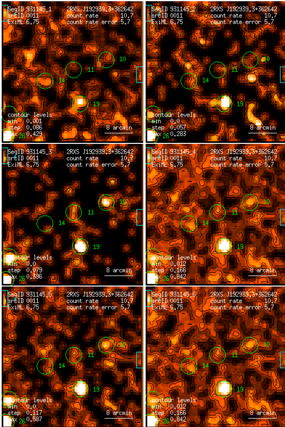
Figure 11: RASS 931145: detection 0011: band rate images, Gaussian filter: (1) PSPC channels 11 – 41, (2) 52 – 90, (3) 91 – 201, (4) 11 – 235, (5) 52 – 201, (6) 11 – 201. Broad band rates in counts/ks. Band rate contour levels in counts/ks/arcmin 2 .
