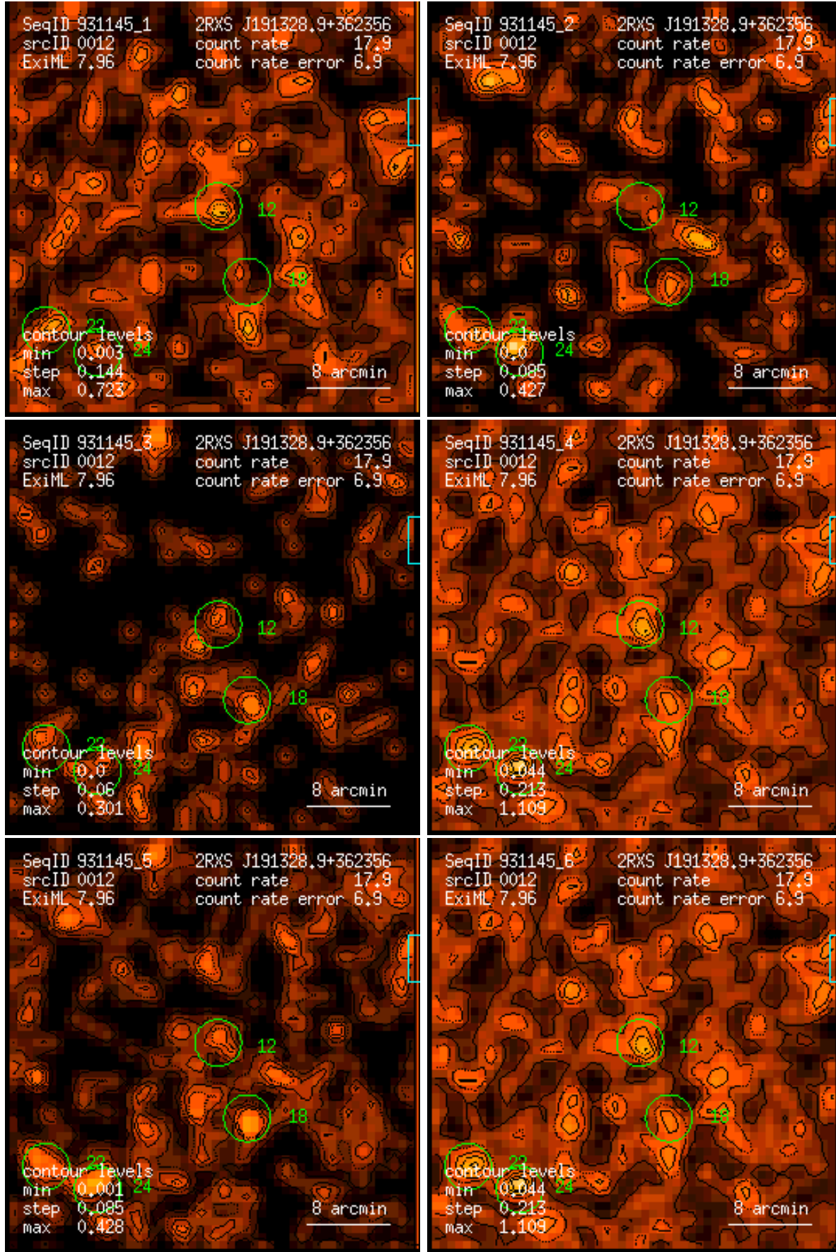
Figure 12: RASS 931145: detection 0012: band rate images, Gaussian filter: (1) PSPC channels 11 – 41, (2) 52 – 90, (3) 91 – 201, (4) 11 – 235, (5) 52 – 201, (6) 11 – 201. Broad band rates in counts/ks. Band rate contour levels in counts/ks/arcmin 2 .
