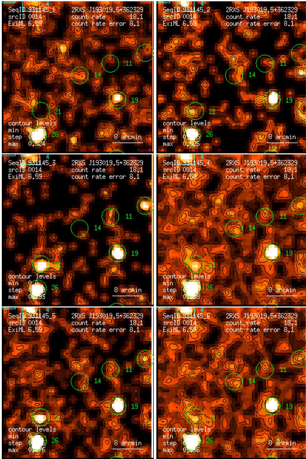
Figure 14: RASS 931145: detection 0014: band rate images, Gaussian filter: (1) PSPC channels 11 – 41, (2) 52 – 90, (3) 91 – 201, (4) 11 – 235, (5) 52 – 201, (6) 11 – 201. Broad band rates in counts/ks. Band rate contour levels in counts/ks/arcmin 2 .
