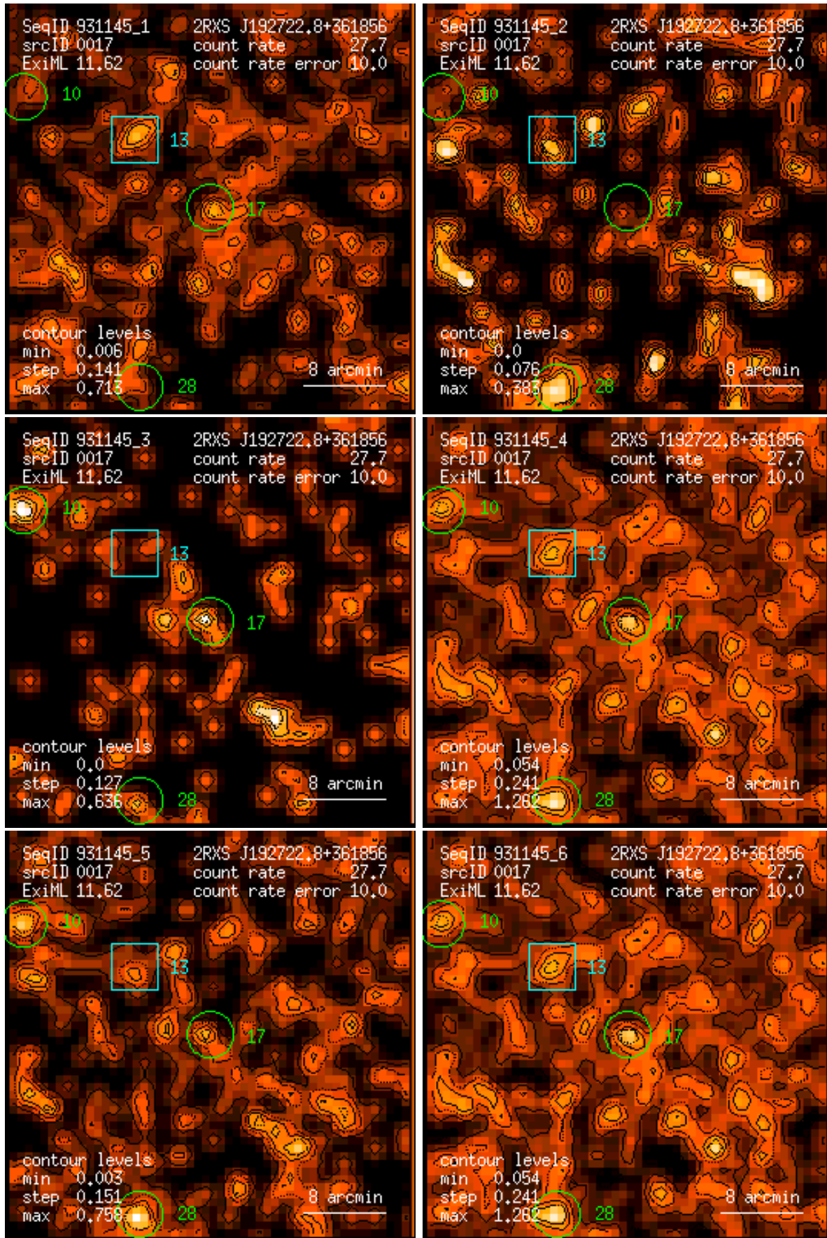
Figure 17: RASS 931145: detection 0017: band rate images, Gaussian filter: (1) PSPC channels 11 – 41, (2) 52 – 90, (3) 91 – 201, (4) 11 – 235, (5) 52 – 201, (6) 11 – 201. Broad band rates in counts/ks. Band rate contour levels in counts/ks/arcmin 2 .
