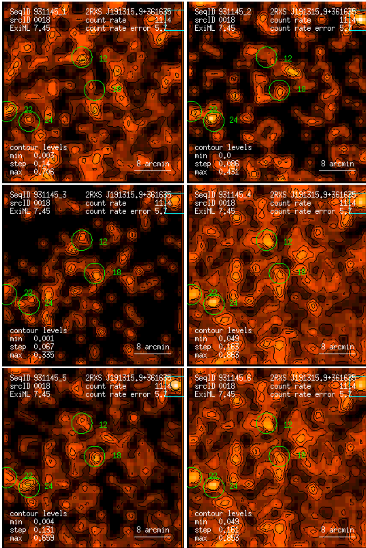
Figure 18: RASS 931145: detection 0018: band rate images, Gaussian filter: (1) PSPC channels 11 – 41, (2) 52 – 90, (3) 91 – 201, (4) 11 – 235, (5) 52 – 201, (6) 11 – 201. Broad band rates in counts/ks. Band rate contour levels in counts/ks/arcmin 2 .
