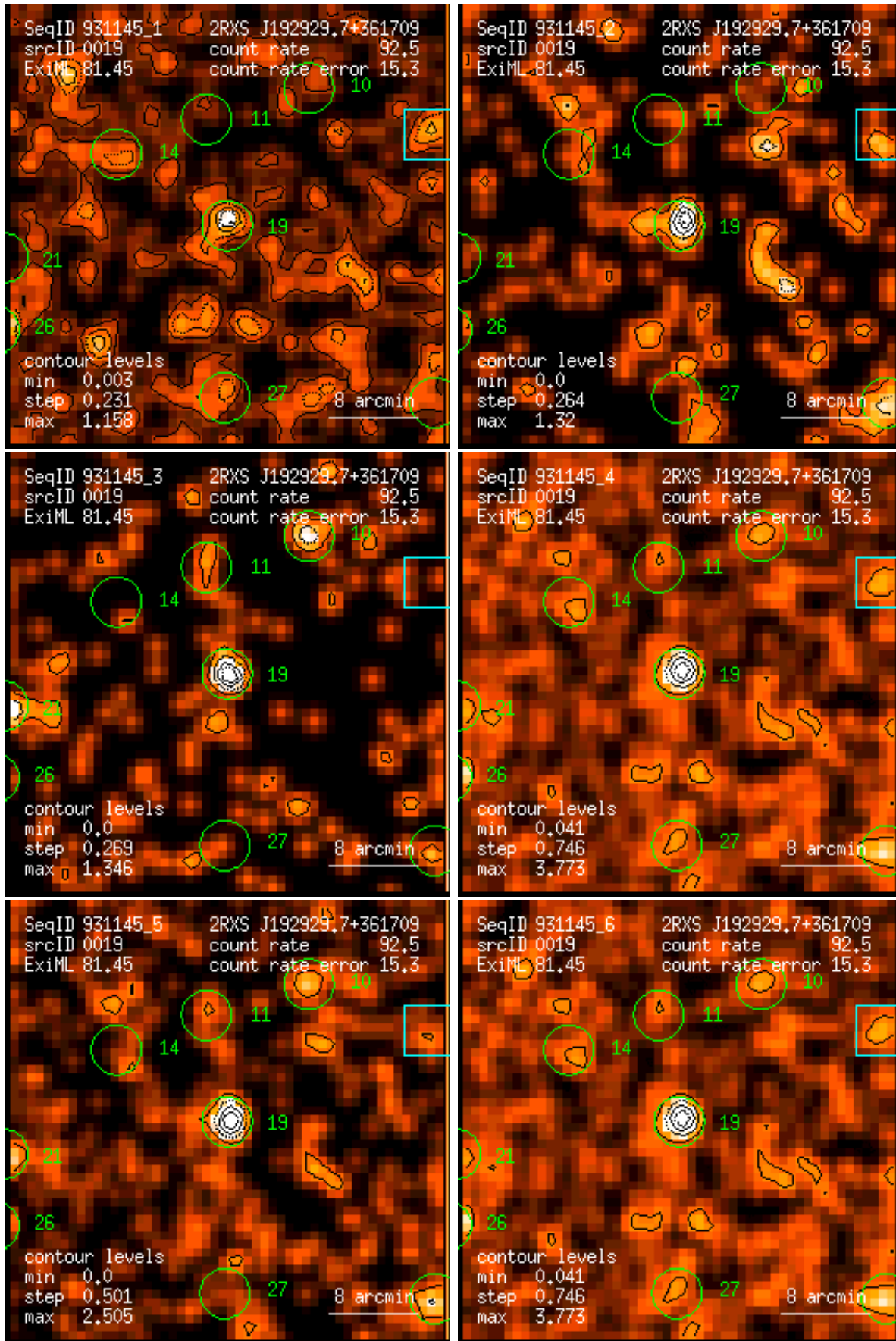
Figure 19: RASS 931145: detection 0019: band rate images, Gaussian filter: (1) PSPC channels 11 – 41, (2) 52 – 90, (3) 91 – 201, (4) 11 – 235, (5) 52 – 201, (6) 11 – 201. Broad band rates in counts/ks. Band rate contour levels in counts/ks/arcmin 2 .
