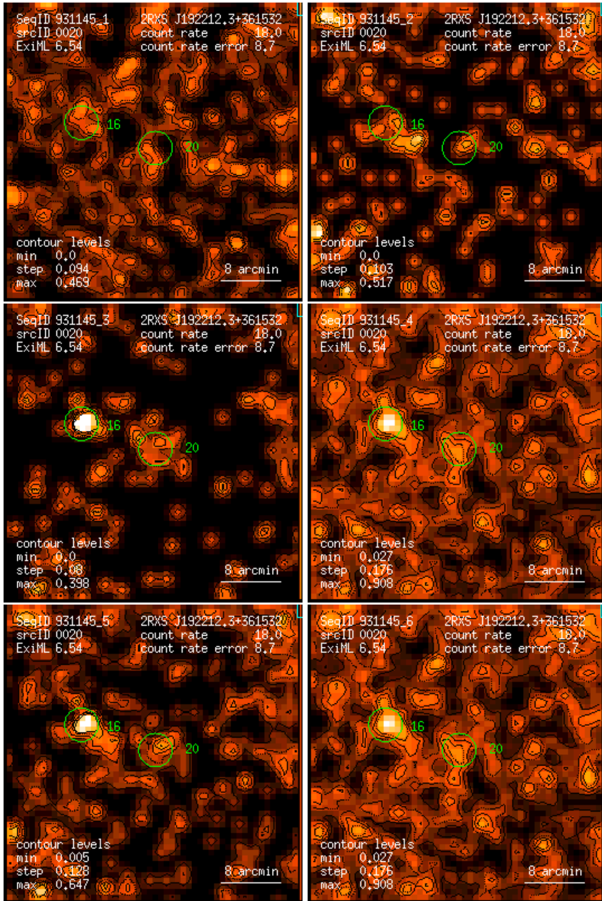
Figure 20: RASS 931145: detection 0020: band rate images, Gaussian filter: (1) PSPC channels 11 – 41, (2) 52 – 90, (3) 91 – 201, (4) 11 – 235, (5) 52 – 201, (6) 11 – 201. Broad band rates in counts/ks. Band rate contour levels in counts/ks/arcmin 2 .
