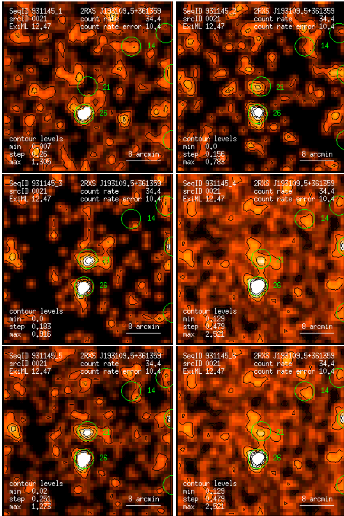
Figure 21: RASS 931145: detection 0021: band rate images, Gaussian filter: (1) PSPC channels 11 – 41, (2) 52 – 90, (3) 91 – 201, (4) 11 – 235, (5) 52 – 201, (6) 11 – 201. Broad band rates in counts/ks. Band rate contour levels in counts/ks/arcmin 2 .
