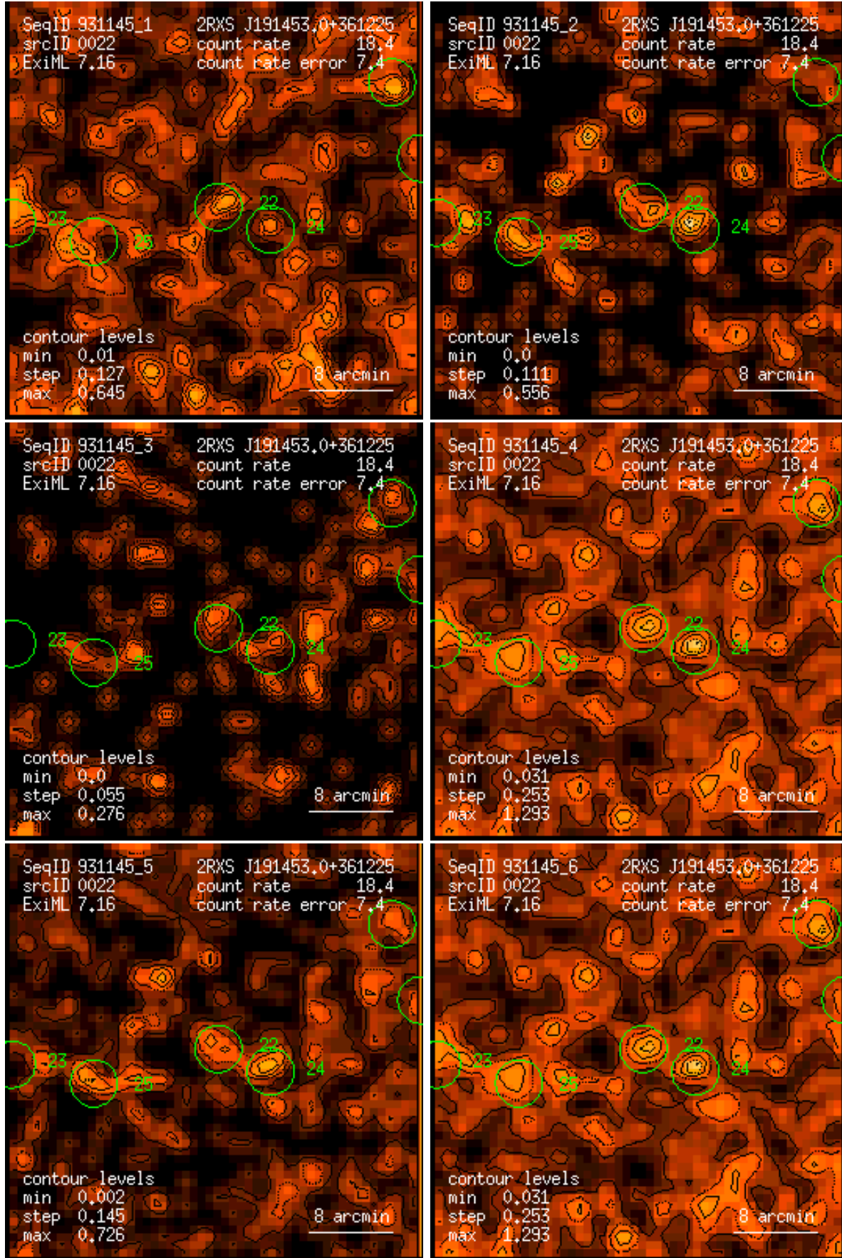
Figure 22: RASS 931145: detection 0022: band rate images, Gaussian filter: (1) PSPC channels 11 – 41, (2) 52 – 90, (3) 91 – 201, (4) 11 – 235, (5) 52 – 201, (6) 11 – 201. Broad band rates in counts/ks. Band rate contour levels in counts/ks/arcmin 2 .
