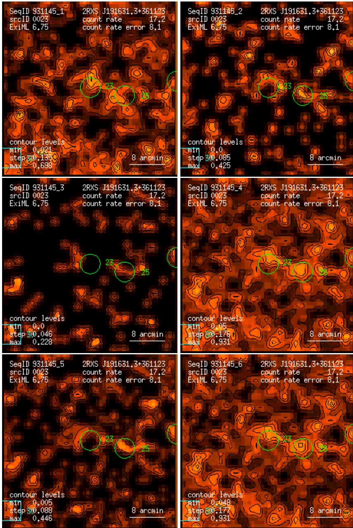
Figure 23: RASS 931145: detection 0023: band rate images, Gaussian filter: (1) PSPC channels 11 – 41, (2) 52 – 90, (3) 91 – 201, (4) 11 – 235, (5) 52 – 201, (6) 11 – 201. Broad band rates in counts/ks. Band rate contour levels in counts/ks/arcmin 2 .
