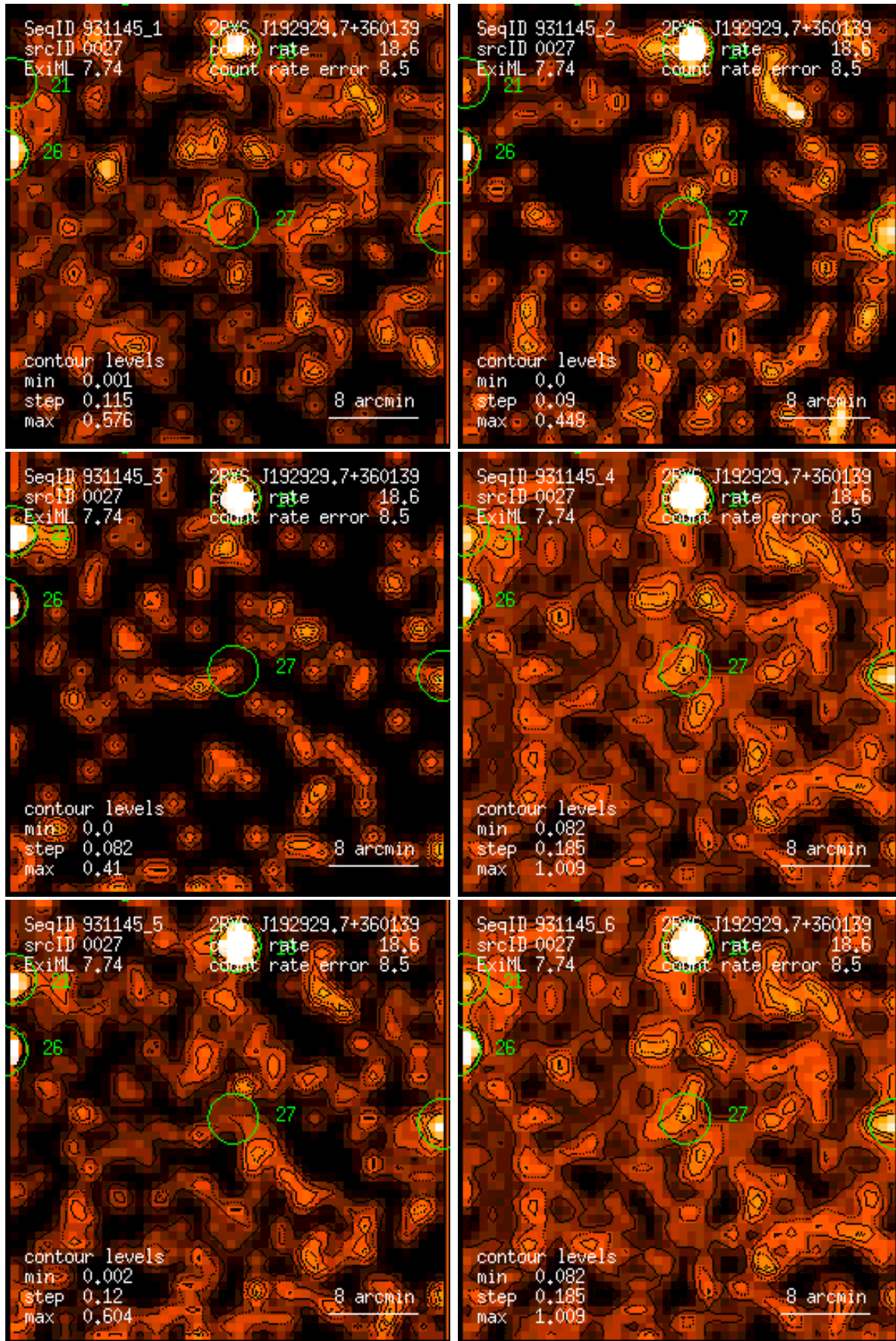
Figure 27: RASS 931145: detection 0027: band rate images, Gaussian filter: (1) PSPC channels 11 – 41, (2) 52 – 90, (3) 91 – 201, (4) 11 – 235, (5) 52 – 201, (6) 11 – 201. Broad band rates in counts/ks. Band rate contour levels in counts/ks/arcmin 2 .
