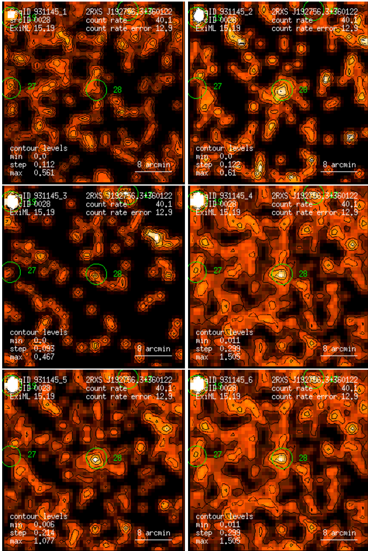
Figure 28: RASS 931145: detection 0028: band rate images, Gaussian filter: (1) PSPC channels 11 – 41, (2) 52 – 90, (3) 91 – 201, (4) 11 – 235, (5) 52 – 201, (6) 11 – 201. Broad band rates in counts/ks. Band rate contour levels in counts/ks/arcmin 2 .
