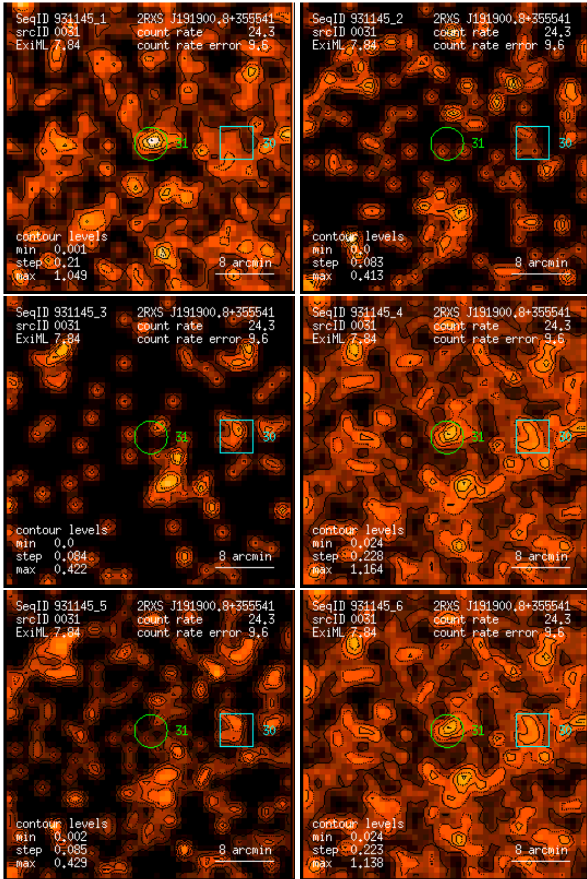
Figure 31: RASS 931145: detection 0031: band rate images, Gaussian filter: (1) PSPC channels 11 – 41, (2) 52 – 90, (3) 91 – 201, (4) 11 – 235, (5) 52 – 201, (6) 11 – 201. Broad band rates in counts/ks. Band rate contour levels in counts/ks/arcmin 2 .
