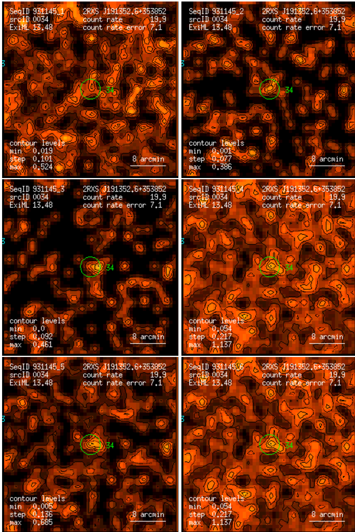
Figure 34: RASS 931145: detection 0034: band rate images, Gaussian filter: (1) PSPC channels 11 – 41, (2) 52 – 90, (3) 91 – 201, (4) 11 – 235, (5) 52 – 201, (6) 11 – 201. Broad band rates in counts/ks. Band rate contour levels in counts/ks/arcmin 2 .
