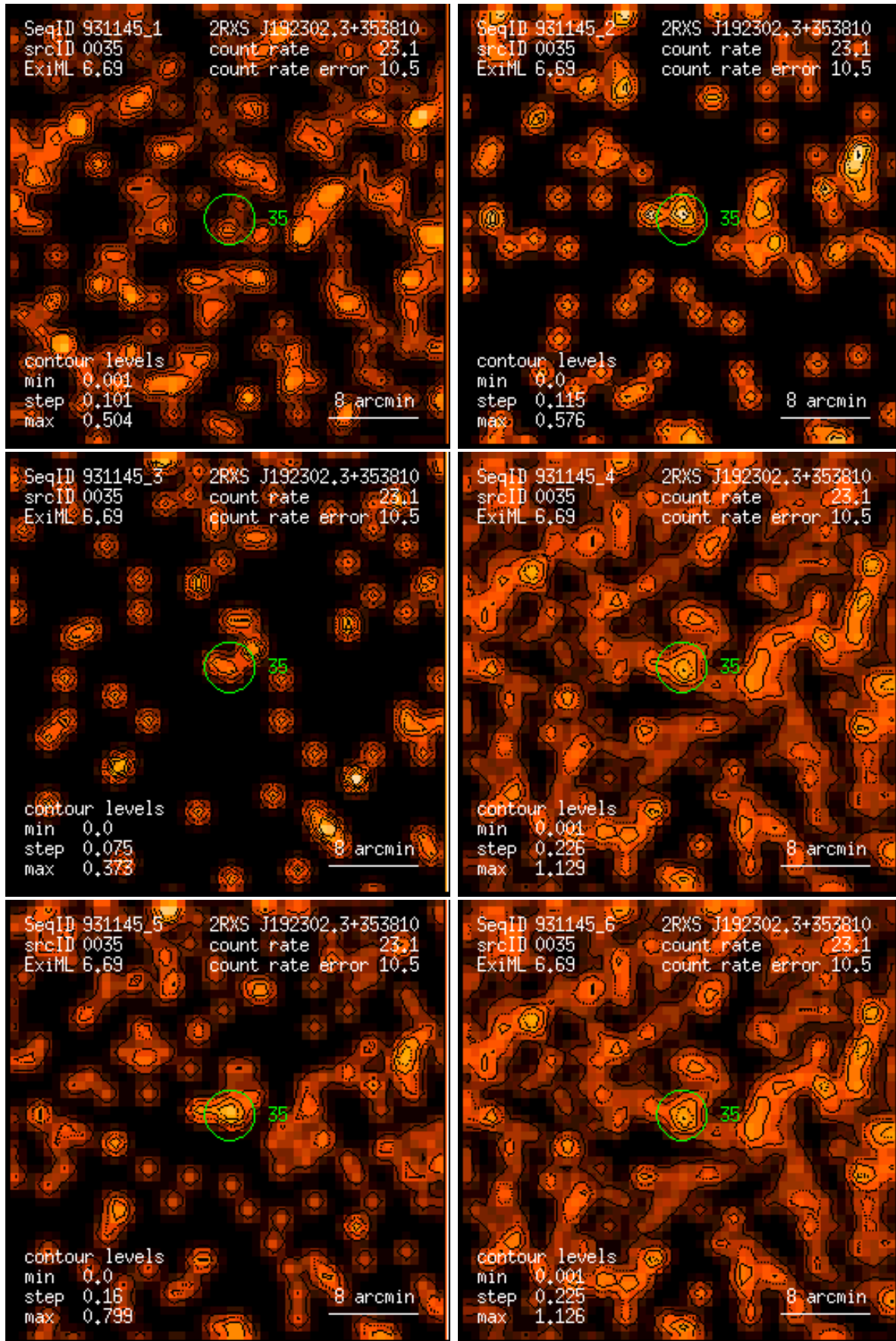
Figure 35: RASS 931145: detection 0035: band rate images, Gaussian filter: (1) PSPC channels 11 – 41, (2) 52 – 90, (3) 91 – 201, (4) 11 – 235, (5) 52 – 201, (6) 11 – 201. Broad band rates in counts/ks. Band rate contour levels in counts/ks/arcmin 2 .
