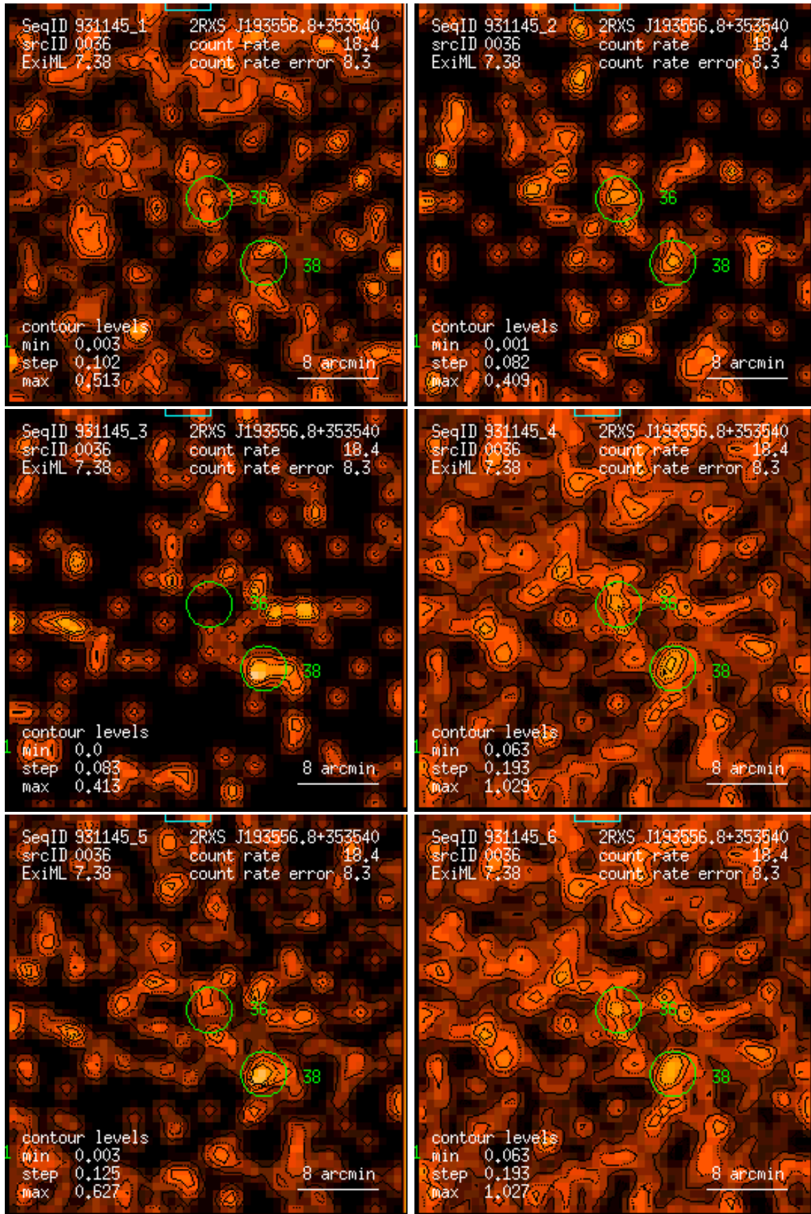
Figure 36: RASS 931145: detection 0036: band rate images, Gaussian filter: (1) PSPC channels 11 – 41, (2) 52 – 90, (3) 91 – 201, (4) 11 – 235, (5) 52 – 201, (6) 11 – 201. Broad band rates in counts/ks. Band rate contour levels in counts/ks/arcmin 2 .
