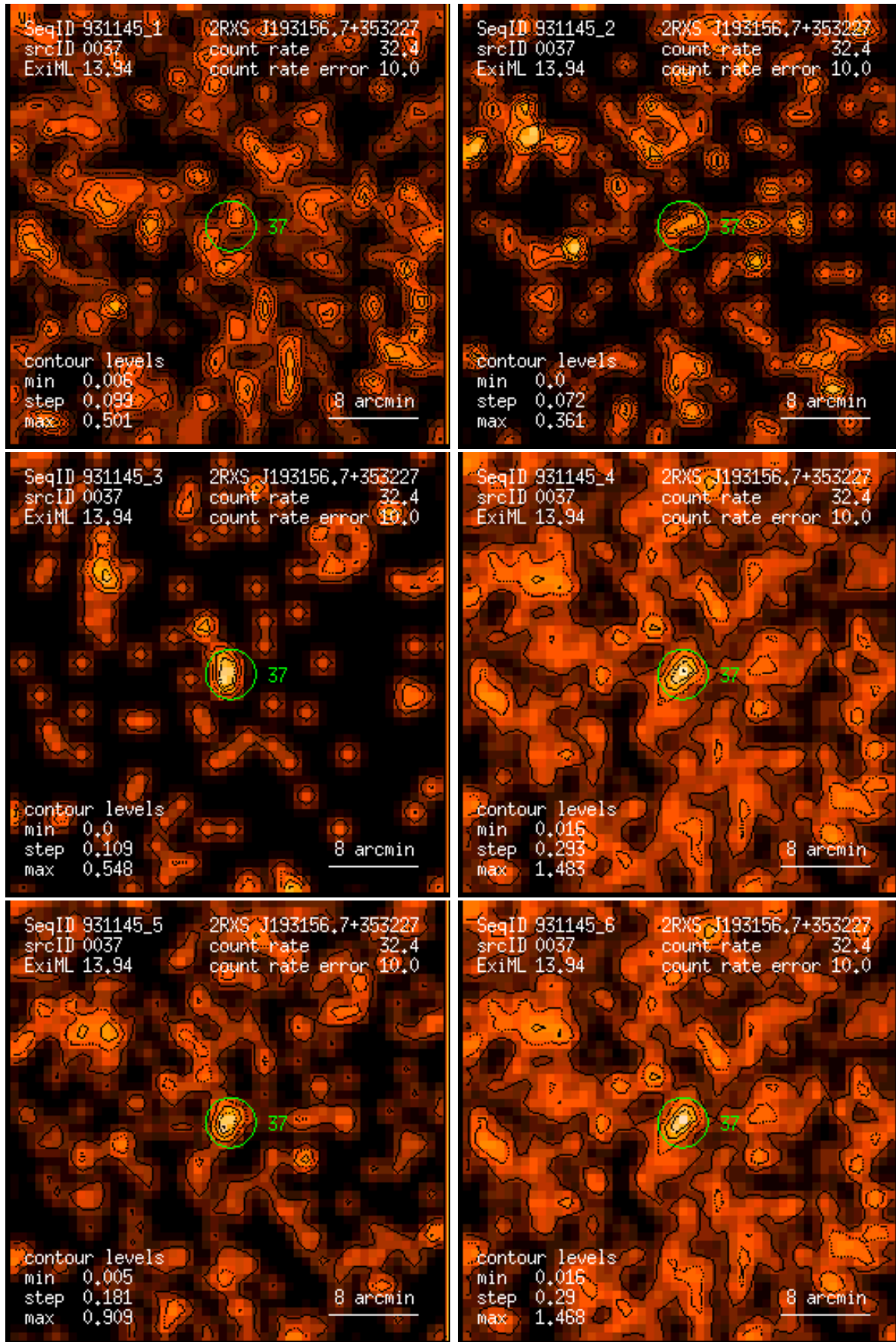
Figure 37: RASS 931145: detection 0037: band rate images, Gaussian filter: (1) PSPC channels 11 – 41, (2) 52 – 90, (3) 91 – 201, (4) 11 – 235, (5) 52 – 201, (6) 11 – 201. Broad band rates in counts/ks. Band rate contour levels in counts/ks/arcmin 2 .
