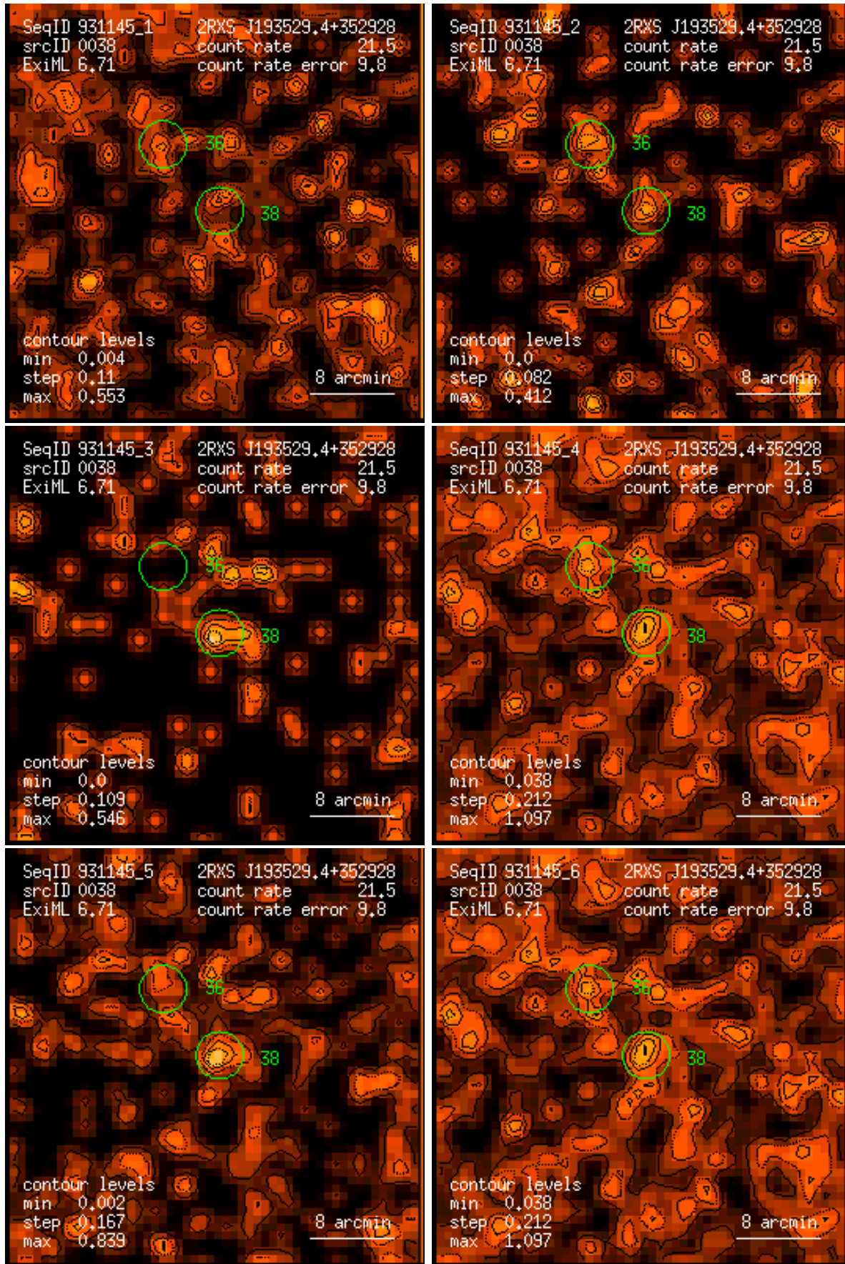
Figure 38: RASS 931145: detection 0038: band rate images, Gaussian filter: (1) PSPC channels 11 – 41, (2) 52 – 90, (3) 91 – 201, (4) 11 – 235, (5) 52 – 201, (6) 11 – 201. Broad band rates in counts/ks. Band rate contour levels in counts/ks/arcmin 2 .
