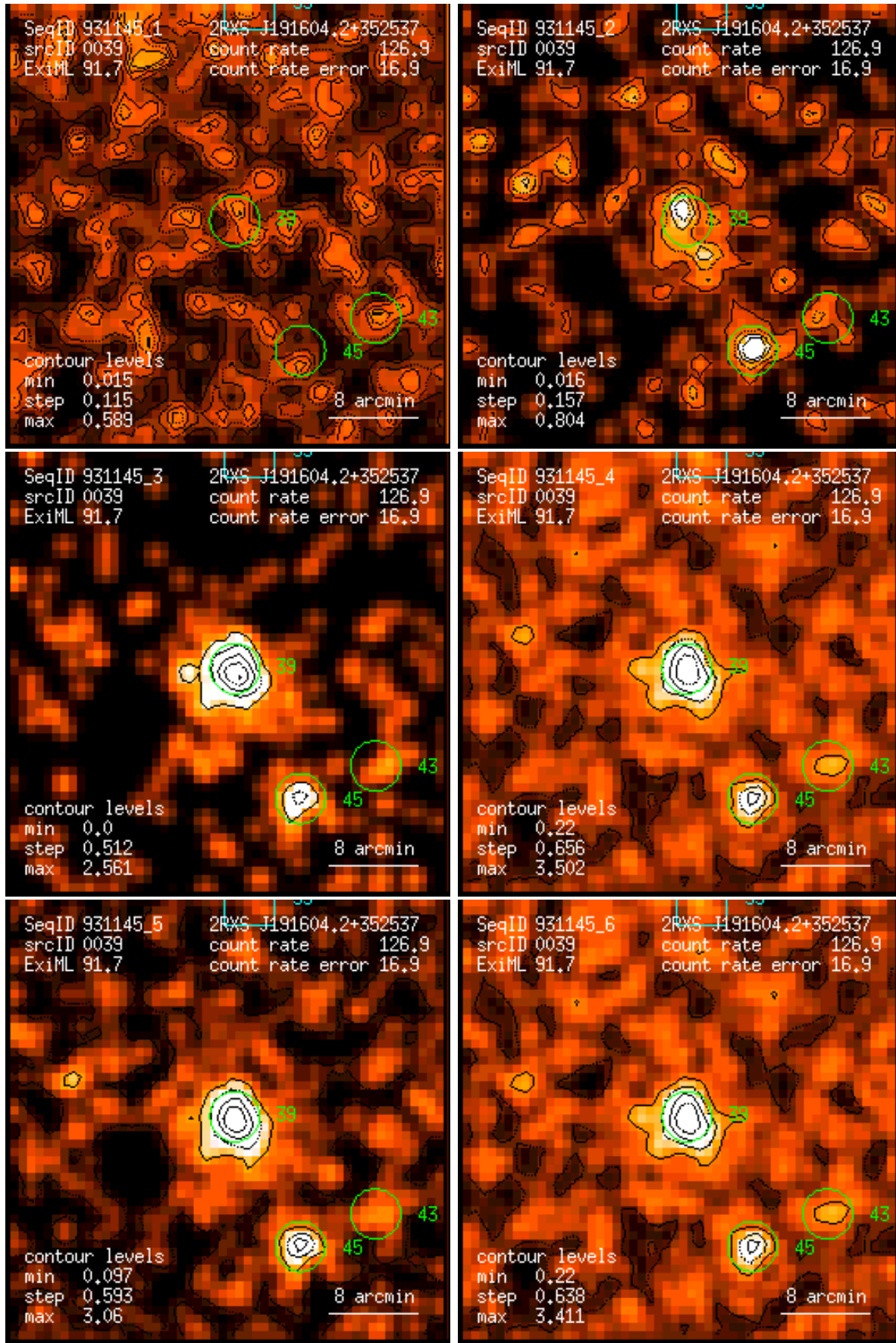
Figure 39: RASS 931145: detection 0039: band rate images, Gaussian filter: (1) PSPC channels 11 – 41, (2) 52 – 90, (3) 91 – 201, (4) 11 – 235, (5) 52 – 201, (6) 11 – 201. Broad band rates in counts/ks. Band rate contour levels in counts/ks/arcmin 2 .
